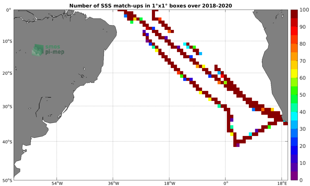
Figure 4: Number of SSS match-ups between TSG (SAMOS) SSS and the SMAP SSS L3 v4 - 8-Day running (RSS) SSS product for the South Atlantic Ocean Pi-MEP region over 1^\circ \times 1^\circ boxes and for the full satellite product period.
