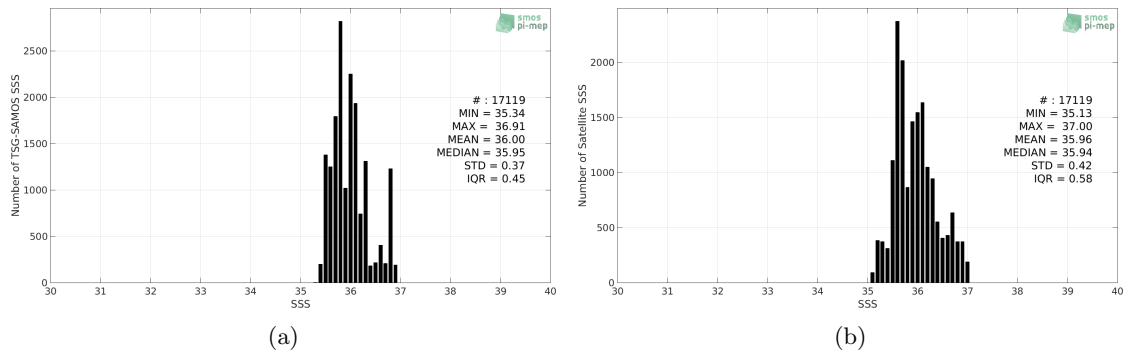
Figure 2: Histograms of SSS from TSG-SAMOS (a) and SMAP-L3-RSS-V4-8DAY-RUNNING (b) considering all match-up pairs per bins of 0.1 over the South Atlantic Ocean Pi-MEP region and for the full satellite product period.
