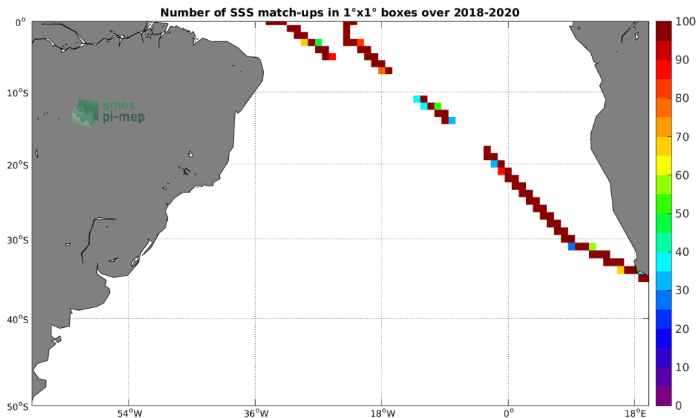
Figure 4: Number of SSS match-ups between TSG-SAMOS SSS and the SMAP-L3-RSS-V4-8DAY-RUNNING SSS product for the South Atlantic Ocean Pi-MEP region over 1^{\circ} \times 1^{\circ} boxes and for the full satellite product period.
