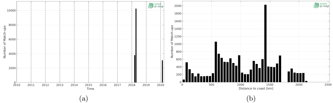
Figure 1: Number of match-ups between TSG-SAMOS and SMAP-L3-RSS-V4-8DAY-RUNNING SSS as a function of time (a) and as function of the distance to coast (b) over the South Atlantic Ocean Pi-MEP region and for the full satellite product period.
