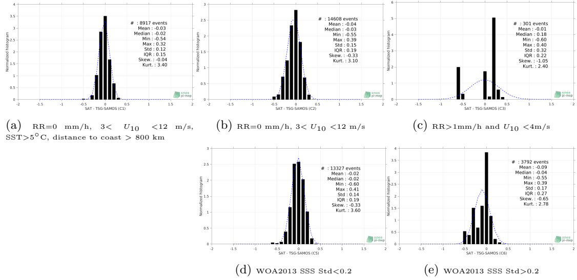
Figure 13: Normalized histogram of \Delta\text{SSS} (SMAP-L3-RSS-V4-8DAY-RUNNING - TSG-SAMOS) for 5 different subdatasets corresponding to: RR=0 mm/h, 3 < U_{10} < 12 m/s, SST > 5^{\circ}\text{C} , distance to coast > 800 km (a), RR=0 mm/h, 3 < U_{10} < 12 m/s (b), RR > 1\text{mm/h} and U_{10} < 4\text{m/s} (c), WOA2013 SSS Std < 0.2 (d), WOA2013 SSS Std > 0.2 (e).
