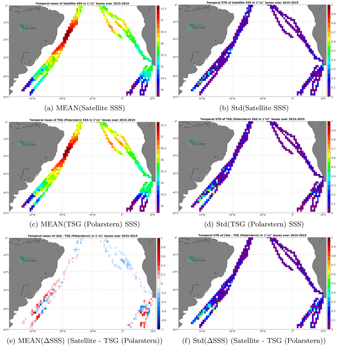
Figure 6: Temporal mean (left) and Std (right) of SSS from SMAP SSS L3 v4 - 8-Day running (RSS) (top), TSG (Polarstern) (middle), and of \Delta SSS (Satellite - TSG (Polarstern)). Only match-up pairs are used to generate these maps.
