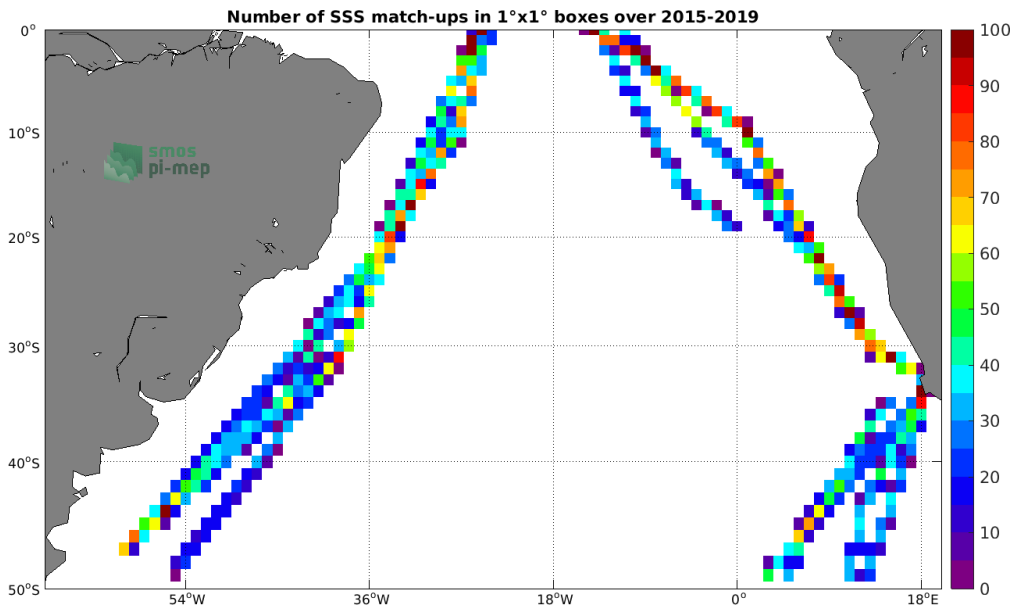
Figure 4: Number of SSS match-ups between TSG (Polarstern) SSS and the SMAP SSS L3 v4 - 8-Day running (RSS) SSS product for the South Atlantic Ocean Pi-MEP region over 1°x1° boxes and for the full satellite product period.
