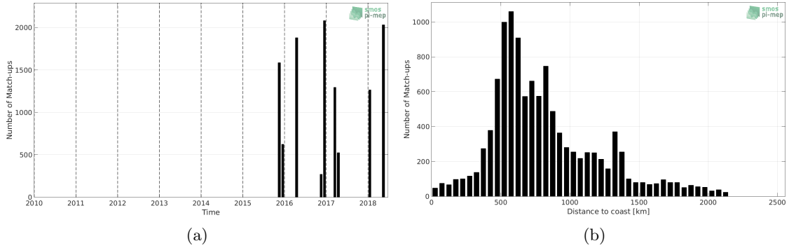
Figure 1: Number of match-ups between TSG-POLARSTERN and SMAP-L3-RSS-V4-8DAY-RUNNING SSS as a function of time (a) and as function of the distance to coast (b) over the South Atlantic Ocean Pi-MEP region and for the full satellite product period.
