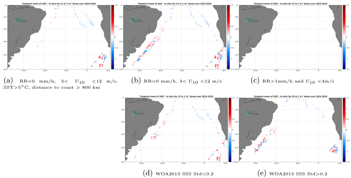
Figure 12: Temporal mean gridded over spatial boxes of size 1^\circ \times 1^\circ of \Delta SSS (SMAP-L3-RSS-V4-8DAY-RUNNING - TSG-POLARSTERN) for 5 different subdatasets corresponding to: RR=0 mm/h, 3 < U_{10} < 12 m/s, SST > 5^\circ C , distance to coast > 800 km (a), RR=0 mm/h, 3 < U_{10} < 12 m/s (b), RR > 1 mm/h and U_{10} < 4 m/s (c), WOA2013 SSS Std < 0.2 (d), WOA2013 SSS Std > 0.2 (e).
