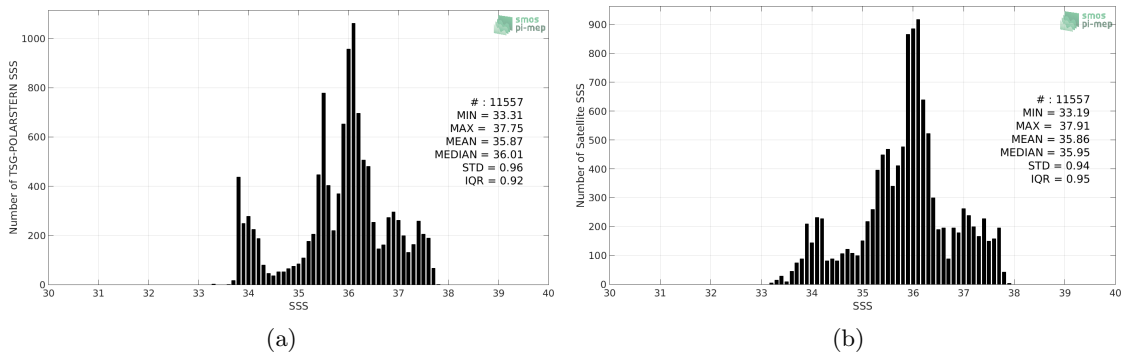
Figure 2: Histograms of SSS from TSG-POLARSTERN (a) and SMAP-L3-RSS-V4-8DAY-RUNNING (b) considering all match-up pairs per bins of 0.1 over the South Atlantic Ocean Pi-MEP region and for the full satellite product period.
