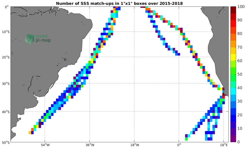
Figure 4: Number of SSS match-ups between TSG-POLARSTERN SSS and the SMAP-L3-RSS-V4-8DAY-RUNNING SSS product for the South Atlantic Ocean Pi-MEP region over 1^\circ \times 1^\circ boxes and for the full satellite product period.
