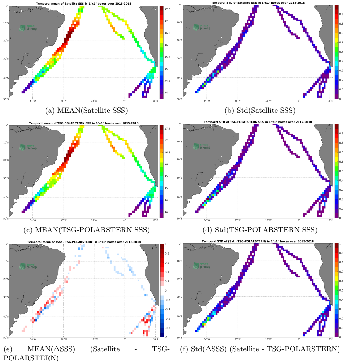
Figure 6: Temporal mean (left) and Std (right) of SSS from SMAP-L3-RSS-V4-8DAY-RUNNING (top), TSG-POLARSTERN (middle), and of \Delta SSS (Satellite - TSG-POLARSTERN). Only match-up pairs are used to generate these maps.
