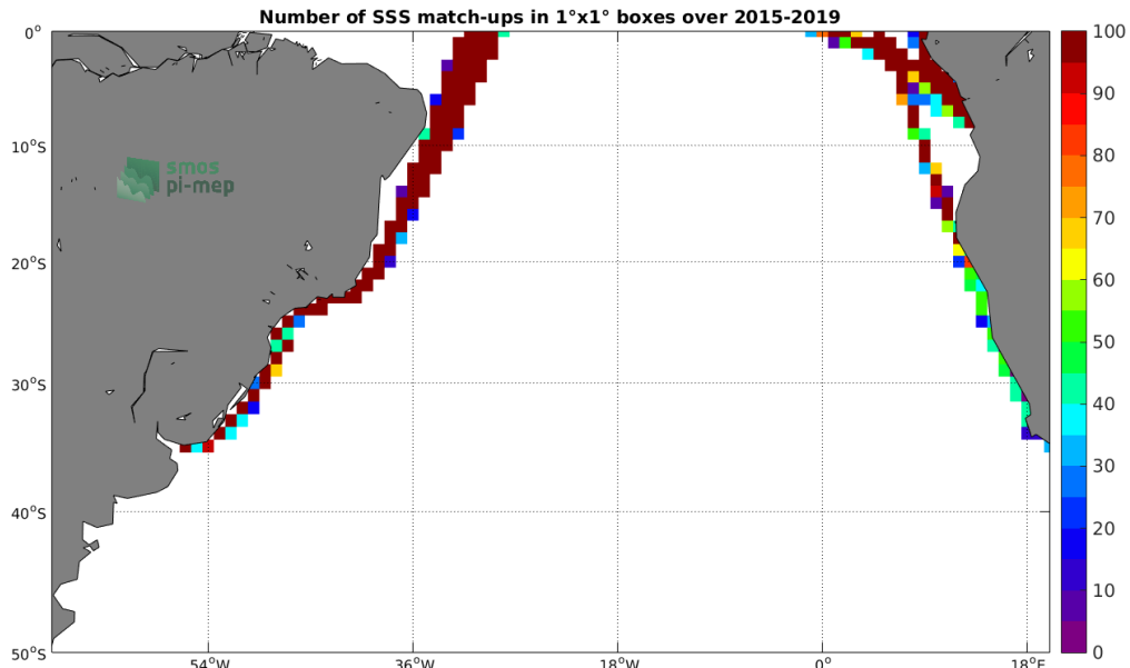
Figure 4: Number of SSS match-ups between TSG (LEGOS-DM) SSS and the SMAP SSS L3 v4 - 8-Day running (RSS) SSS product for the South Atlantic Ocean Pi-MEP region over 1^\circ \times 1^\circ boxes and for the full satellite product period.
