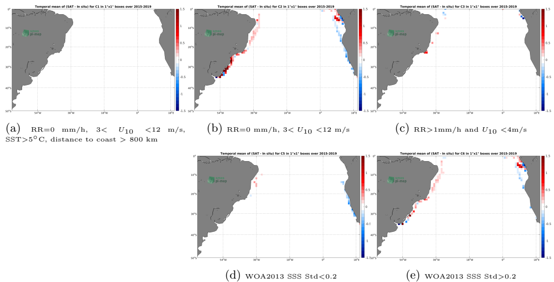
Figure 12: Temporal mean gridded over spatial boxes of size 1^\circ \times 1^\circ of \Delta SSS (SMAP SSS L3 v4 - 8-Day running (RSS) - TSG (LEGOS-DM)) for 5 different subdatasets corresponding to: RR=0 mm/h, 3 < U_{10} < 12 m/s, SST > 5^\circ\text{C} , distance to coast > 800 km (a), RR=0 mm/h, 3 < U_{10} < 12 m/s (b), RR > 1 mm/h and U_{10} < 4 m/s (c), WOA2013 SSS Std < 0.2 (d), WOA2013 SSS Std > 0.2 (e).
