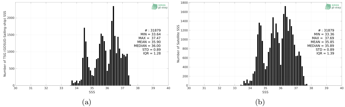
Figure 2: Histograms of SSS from TSG (GOSUD-Sailing-ship) (a) and SMAP SSS L3 v4 - 8-Day running (RSS) (b) considering all match-up pairs per bins of 0.1 over the South Atlantic Ocean Pi-MEP region and for the full satellite product period.
