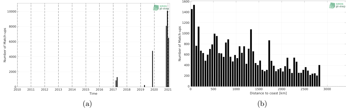
Figure 1: Number of match-ups between TSG (GOSUD-Sailing-ship) and SMAP SSS L3 v4 - 8-Day running (RSS) SSS as a function of time (a) and as function of the distance to coast (b) over the South Atlantic Ocean Pi-MEP region and for the full satellite product period.
