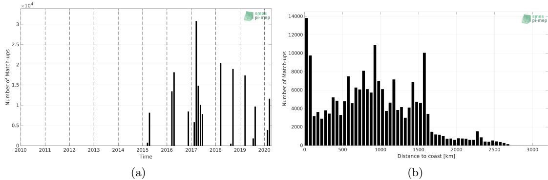
Figure 1: Number of match-ups between TSG (GOSUD-Research-vessel) and SMAP SSS L3 v4 - 8-Day running (RSS) SSS as a function of time (a) and as function of the distance to coast (b) over the South Atlantic Ocean Pi-MEP region and for the full satellite product period.
