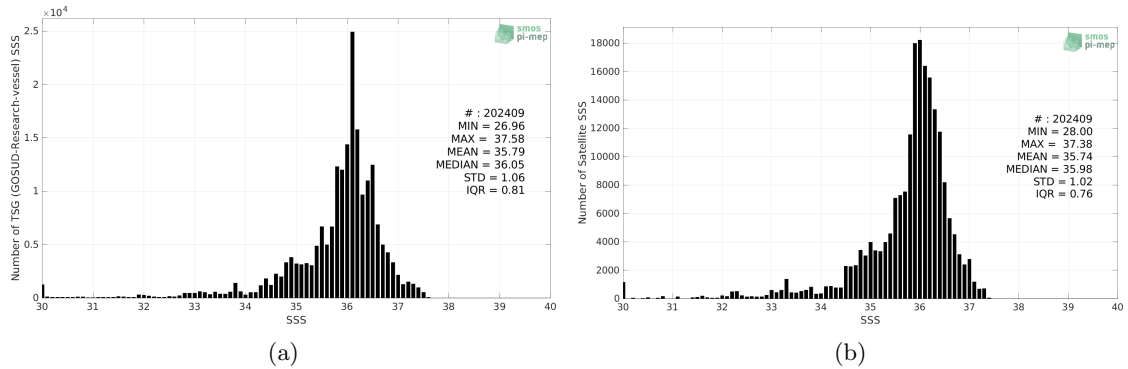
Figure 2: Histograms of SSS from TSG (GOSUD-Research-vessel) (a) and SMAP SSS L3 v4 - 8-Day running (RSS) (b) considering all match-up pairs per bins of 0.1 over the South Atlantic Ocean Pi-MEP region and for the full satellite product period.
