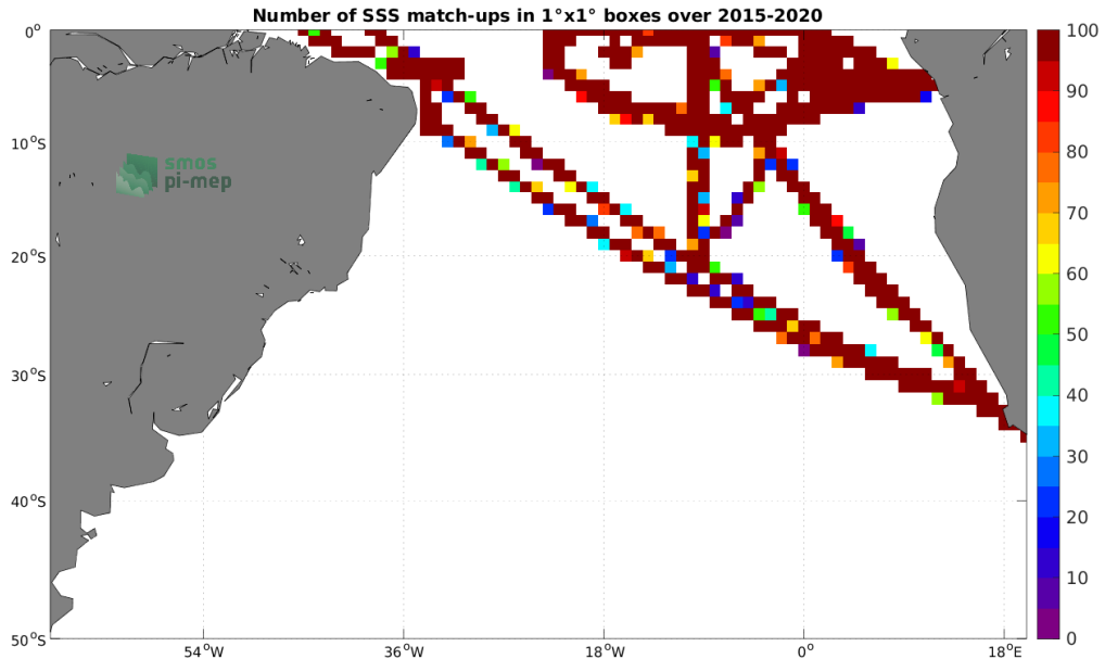
Figure 4: Number of SSS match-ups between TSG (GOSUD-Research-vessel) SSS and the SMAP SSS L3 v4 - 8-Day running (RSS) SSS product for the South Atlantic Ocean Pi-MEP region over 1^\circ \times 1^\circ boxes and for the full satellite product period.
