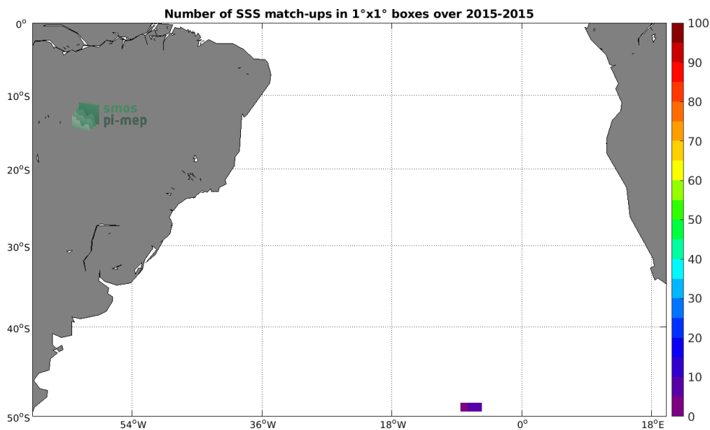
Figure 4: Number of SSS match-ups between Sea mammals SSS and the SMAP SSS L3 v4 - 8-Day running (RSS) SSS product for the South Atlantic Ocean Pi-MEP region over 1°x1° boxes and for the full satellite product period.
