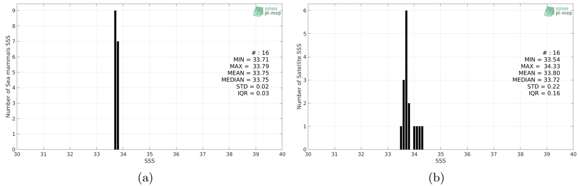
Figure 2: Histograms of SSS from Sea mammals (a) and SMAP SSS L3 v4 - 8-Day running (RSS) (b) considering all match-up pairs per bins of 0.1 over the South Atlantic Ocean Pi-MEP region and for the full satellite product period.
