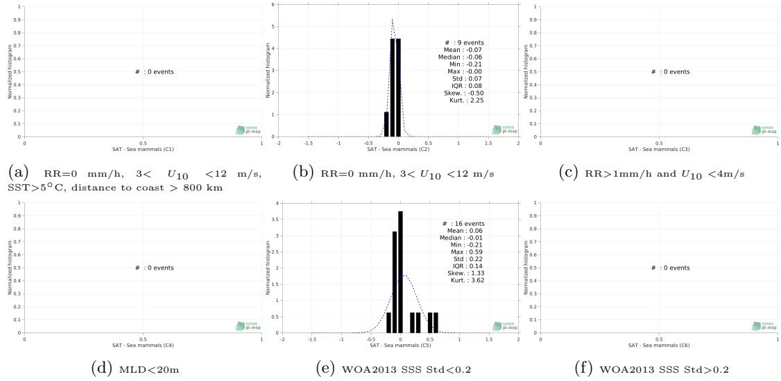
Figure 13: Normalized histogram of \Delta SSS (SMAP SSS L3 v4 - 8-Day running (RSS) - Sea mammals) for 6 different subdatasets corresponding to: RR=0 mm/h, 3 < U_{10} < 12 m/s, SST >5^{\circ} C, distance to coast > 800 km (a), RR=0 mm/h, 3 < U_{10} < 12 m/s (b), RR >1 mm/h and U_{10} < 4 m/s (c), MLD <20 m (d), WOA2013 SSS Std <0.2 (e), WOA2013 SSS Std >0.2 (f).
