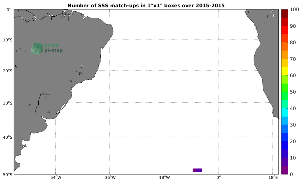
Figure 4: Number of SSS match-ups between Sea mammals SSS and the SMAP SSS L3 v4 - 8-Day running (RSS) SSS product for the South Atlantic Ocean Pi-MEP region over 1^\circ \times 1^\circ boxes and for the full satellite product period.
