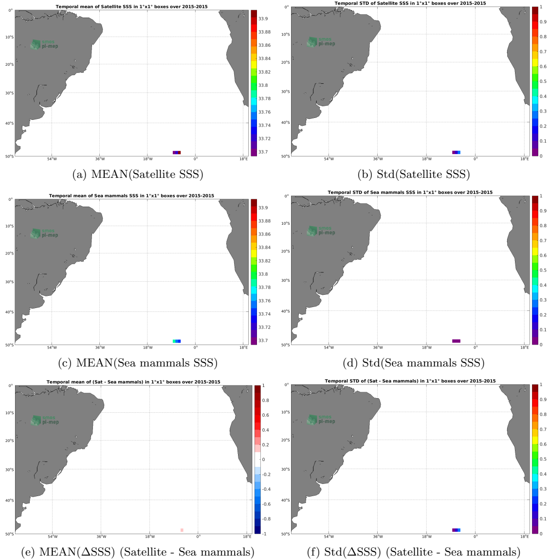
Figure 6: Temporal mean (left) and Std (right) of SSS from SMAP SSS L3 v4 - 8-Day running (RSS) (top), Sea mammals (middle), and of \Delta SSS (Satellite - Sea mammals). Only match-up pairs are used to generate these maps.
