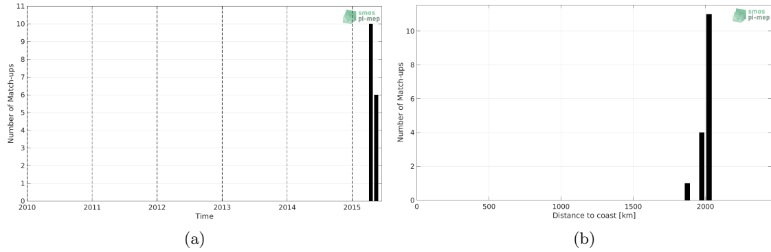
Figure 1: Number of match-ups between Sea mammals and SMAP SSS L3 v4 - 8-Day running (RSS) SSS as a function of time (a) and as function of the distance to coast (b) over the South Atlantic Ocean Pi-MEP region and for the full satellite product period.
