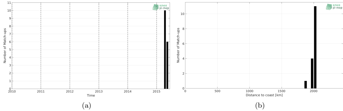
Figure 1: Number of match-ups between Sea mammals and SMAP-L3-RSS-V4-8DAY-RUNNING SSS as a function of time (a) and as function of the distance to coast (b) over the South Atlantic Ocean Pi-MEP region and for the full satellite product period.
