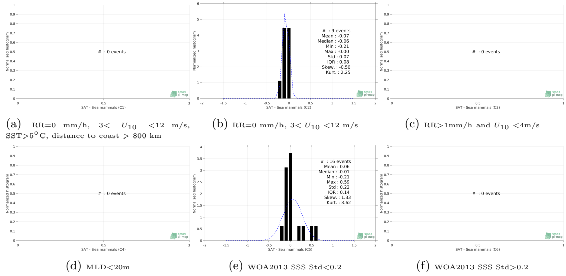
Figure 13: Normalized histogram of \Delta SSS (SMAP-L3-RSS-V4-8DAY-RUNNING - Sea mammals) for 6 different subdatasets corresponding to: RR=0 mm/h, 3 < U_{10} < 12 m/s, SST>5°C, distance to coast > 800 km (a), RR=0 mm/h, 3 < U_{10} < 12 m/s (b), RR>1mm/h and U_{10} < 4 m/s (c), MLD<20m (d), WOA2013 SSS Std<0.2 (e), WOA2013 SSS Std>0.2 (f).
