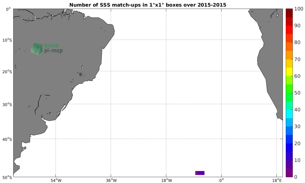
Figure 4: Number of SSS match-ups between Sea mammals SSS and the SMAP-L3-RSS-V4-8DAY-RUNNING SSS product for the South Atlantic Ocean Pi-MEP region over 1^\circ \times 1^\circ boxes and for the full satellite product period.
