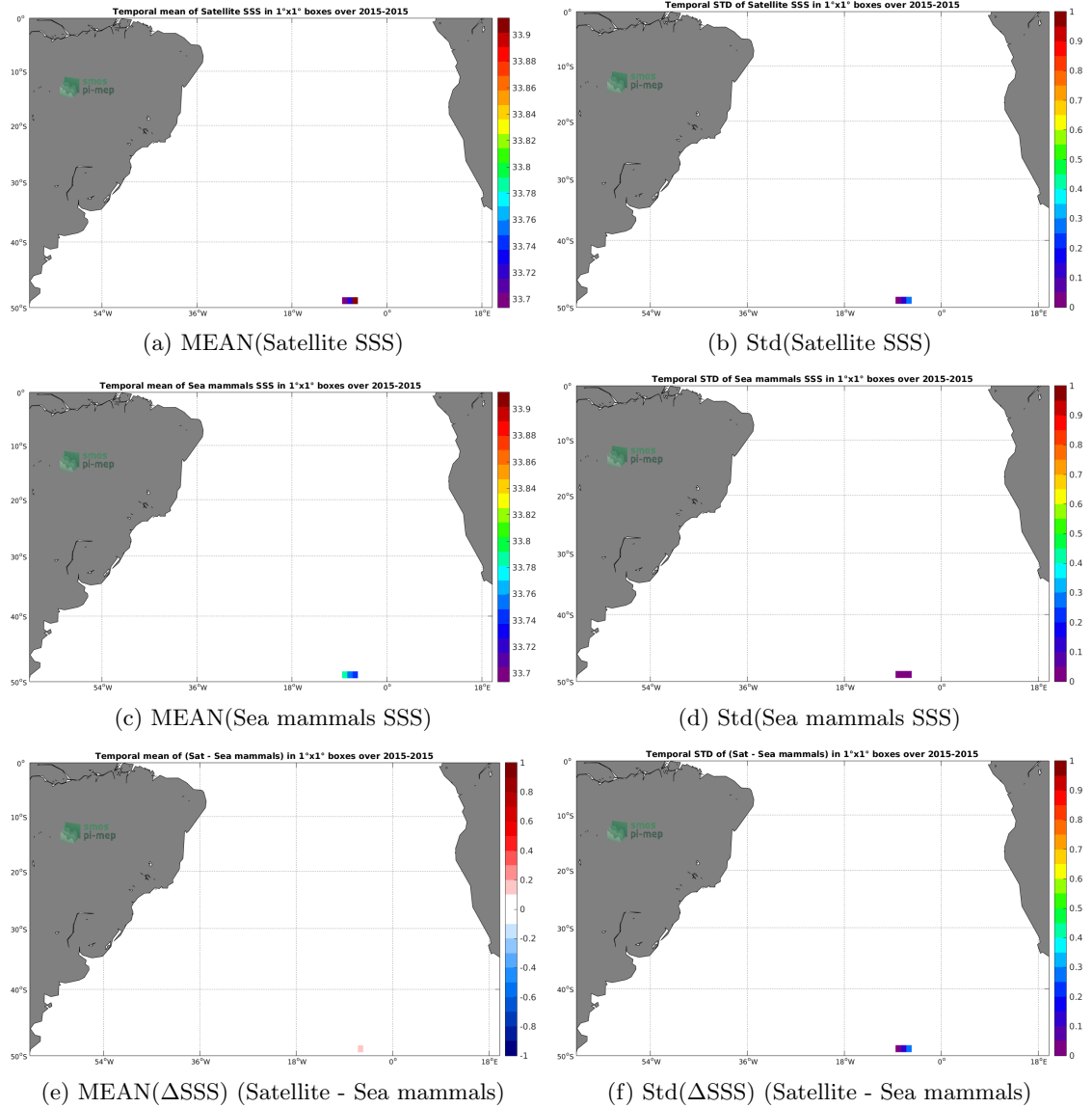
Figure 6: Temporal mean (left) and Std (right) of SSS from SMAP-L3-RSS-V4-8DAY-RUNNING (top), Sea mammals (middle), and of \Delta SSS (Satellite - Sea mammals). Only match-up pairs are used to generate these maps.
