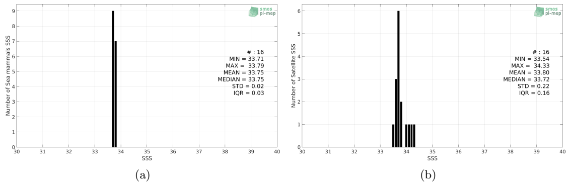
Figure 2: Histograms of SSS from Sea mammals (a) and SMAP-L3-RSS-V4-8DAY-RUNNING (b) considering all match-up pairs per bins of 0.1 over the South Atlantic Ocean Pi-MEP region and for the full satellite product period.
