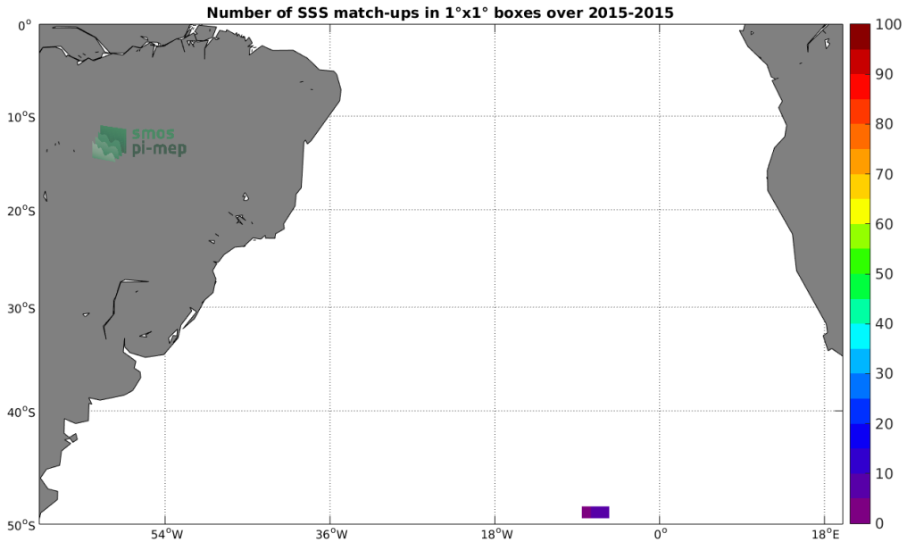
Figure 4: Number of SSS match-ups between Sea mammals SSS and the SMAP-L3-RSS-V4-8DAY-RUNNING SSS product for the South Atlantic Ocean Pi-MEP region over 1^{\circ} \times 1^{\circ} boxes and for the full satellite product period.
