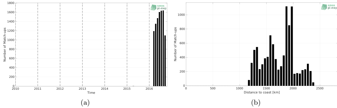
Figure 1: Number of match-ups between Surface drifters and SMAP SSS L3 v4 - 8-Day running (RSS) SSS as a function of time (a) and as function of the distance to coast (b) over the South Atlantic Ocean Pi-MEP region and for the full satellite product period.
