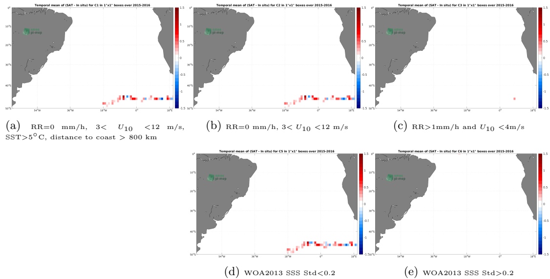
Figure 11: Temporal mean gridded over spatial boxes of size 1^{\circ}\times 1^{\circ} of \Delta\text{SSS} (SMAP SSS L3 v4 - 8-Day running (RSS) - Surface drifters) for 5 different subdatasets corresponding to:RR=0 mm/h, 3 < U_{10} < 12 m/s, SST >5^{\circ}\text{C} , distance to coast > 800 km (a), RR=0 mm/h, 3 < U_{10} < 12 m/s (b), RR >1 mm/h and U_{10} < 4 m/s (c), WOA2013 SSS Std <0.2 (d), WOA2013 SSS Std >0.2 (e).
