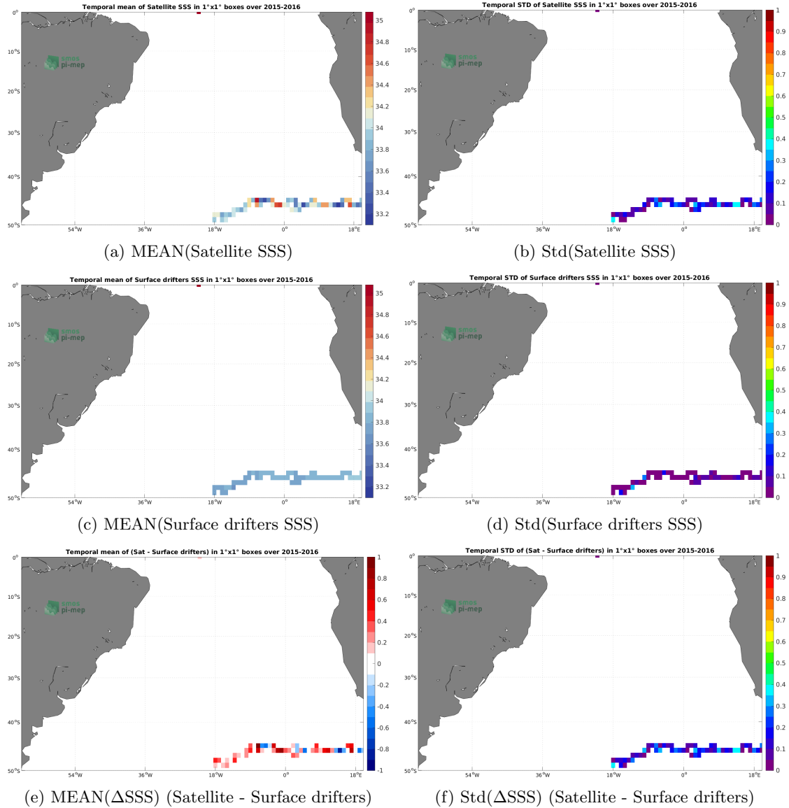
Figure 5: Temporal mean (left) and Std (right) of SSS from SMAP SSS L3 v4 - 8-Day running (RSS) (top), Surface drifters (middle), and of \Delta SSS (Satellite - Surface drifters). Only match-up pairs are used to generate these maps.
