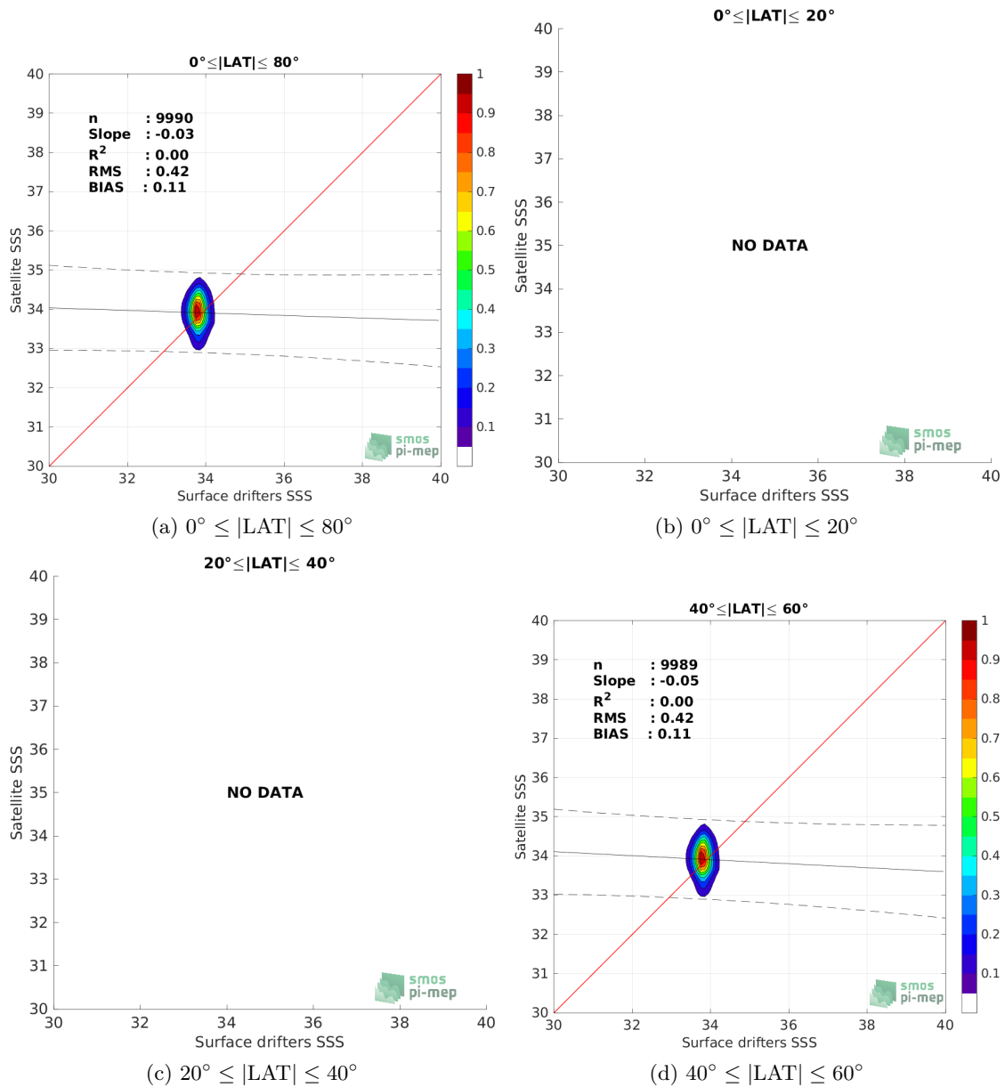
Figure 8: Contour maps of the concentration of SMAP SSS L3 v4 - 8-Day running (RSS) SSS (y-axis) versus Surface drifters SSS (x-axis) at match-up pairs for different latitude bands. For each plot, the red line shows x=y . The black thin and dashed lines indicate a linear fit through the data cloud and the \pm 95\% confidence levels, respectively. The number match-up pairs n , the slope and R^2 coefficient of the linear fit, the root mean square (RMS) and the mean bias between satellite and in situ data are indicated for each latitude band in each plots.
