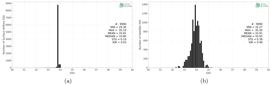
Figure 2: Histograms of SSS from Surface drifters (a) and SMAP SSS L3 v4 - 8-Day running (RSS) (b) considering all match-up pairs per bins of 0.1 over the South Atlantic Ocean Pi-MEP region and for the full satellite product period.
