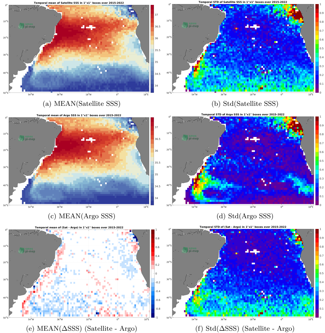
Figure 6: Temporal mean (left) and Std (right) of SSS from SMAP SSS L3 v4 - 8-Day running (RSS) (top), Argo (middle), and of \Delta SSS (Satellite - Argo). Only match-up pairs are used to generate these maps.
