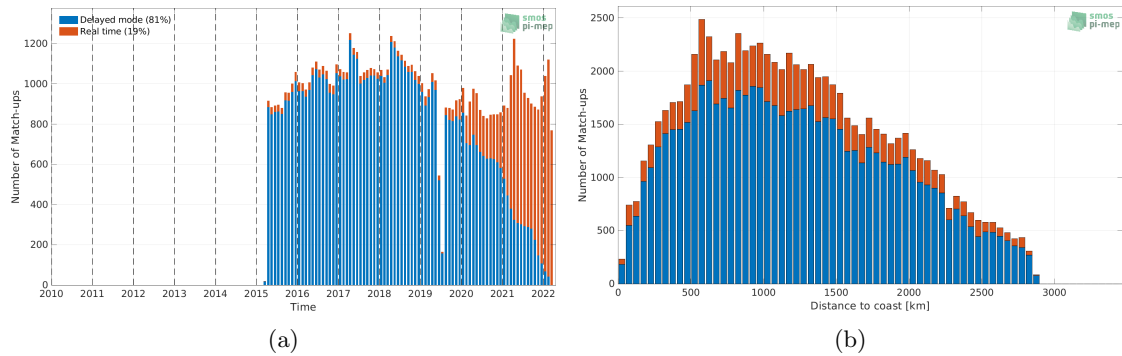
Figure 1: Number of match-ups between Argo and SMAP SSS L3 v4 - 8-Day running (RSS) SSS as a function of time (a) and as function of the distance to coast (b) over the South Atlantic Ocean Pi-MEP region and for the full satellite product period.
