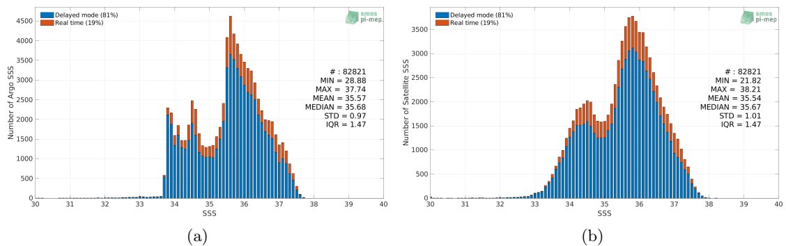
Figure 2: Histograms of SSS from Argo (a) and SMAP SSS L3 v4 - 8-Day running (RSS) (b) considering all match-up pairs per bins of 0.1 over the South Atlantic Ocean Pi-MEP region and for the full satellite product period.
