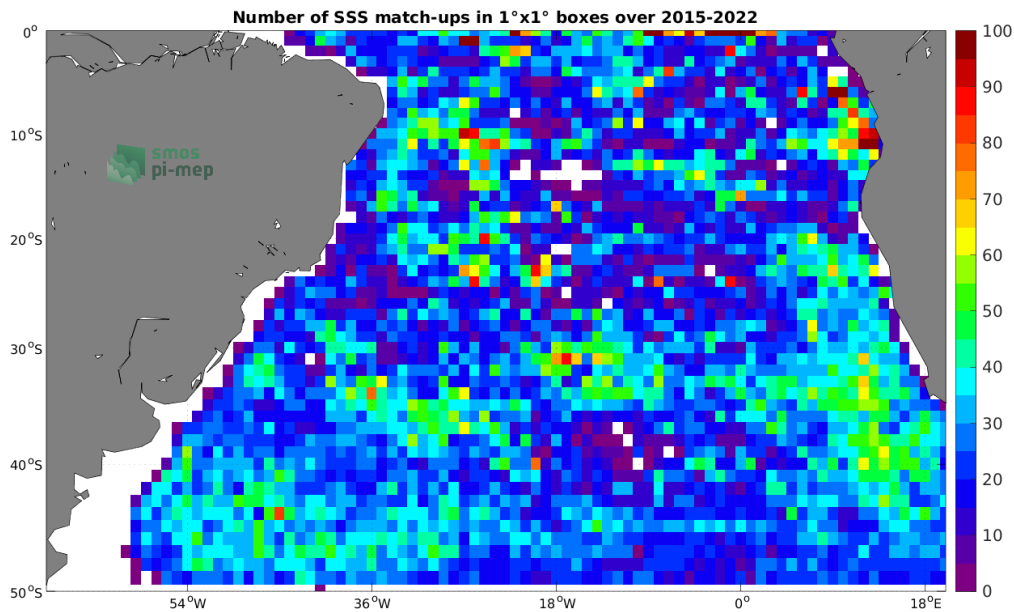
Figure 4: Number of SSS match-ups between Argo SSS and the SMAP SSS L3 v4 - 8-Day running (RSS) SSS product for the South Atlantic Ocean Pi-MEP region over 1^\circ \times 1^\circ boxes and for the full satellite product period.
