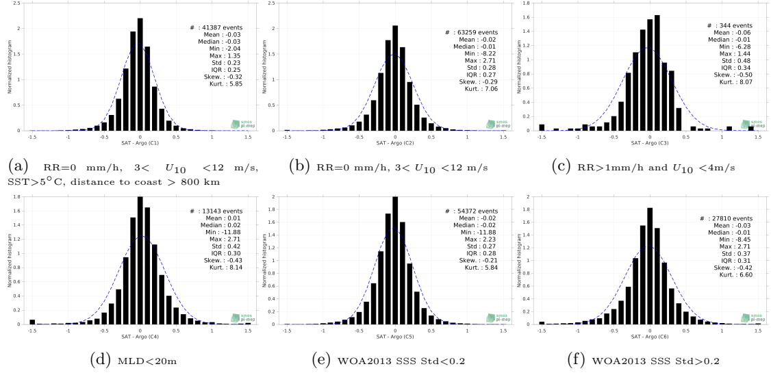
Figure 13: Normalized histogram of \Delta SSS (SMAP SSS L3 v4 - 8-Day running (RSS) - Argo) for 6 different subdatasets corresponding to: RR=0 mm/h, 3 < U_{10} < 12 m/s, SST > 5°C, distance to coast > 800 km (a), RR=0 mm/h, 3 < U_{10} < 12 m/s (b), RR > 1mm/h and U_{10} < 4 m/s (c), MLD < 20m (d), WOA2013 SSS Std < 0.2 (e), WOA2013 SSS Std > 0.2 (f).
