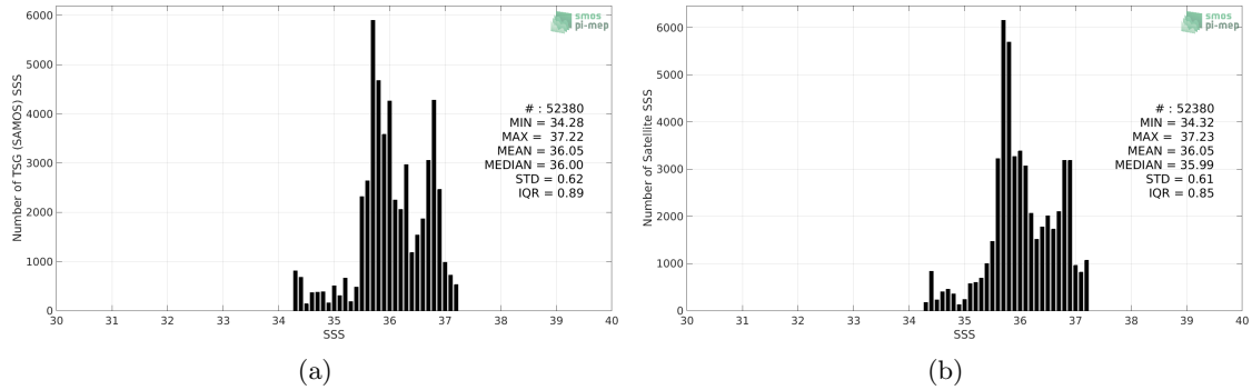
Figure 2: Histograms of SSS from TSG (SAMOS) (a) and SMAP SSS L3 v4 - Monthly (RSS) (b) considering all match-up pairs per bins of 0.1 over the South Atlantic Ocean Pi-MEP region and for the full satellite product period.
