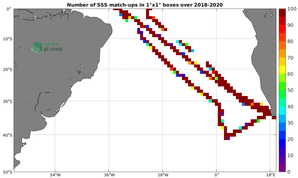
Figure 4: Number of SSS match-ups between TSG (SAMOS) SSS and the SMAP SSS L3 v4 - Monthly (RSS) SSS product for the South Atlantic Ocean Pi-MEP region over 1^\circ \times 1^\circ boxes and for the full satellite product period.
