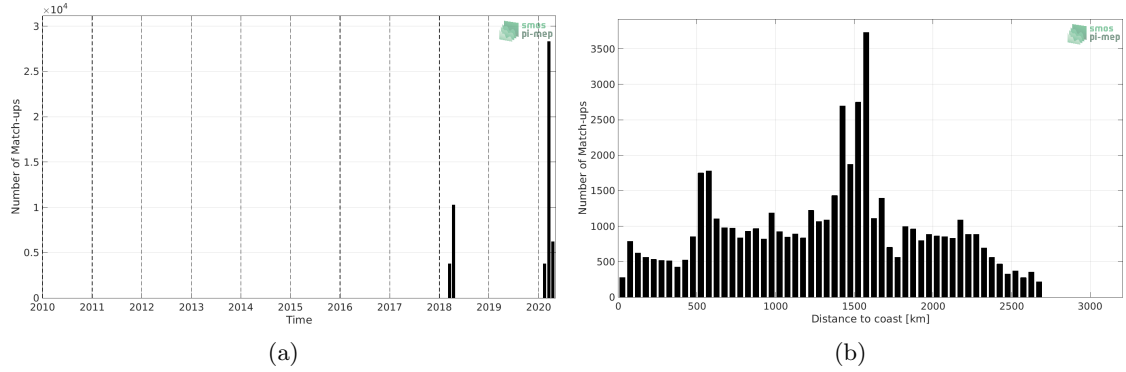
Figure 1: Number of match-ups between TSG (SAMOS) and SMAP SSS L3 v4 - Monthly (RSS) SSS as a function of time (a) and as function of the distance to coast (b) over the South Atlantic Ocean Pi-MEP region and for the full satellite product period.
