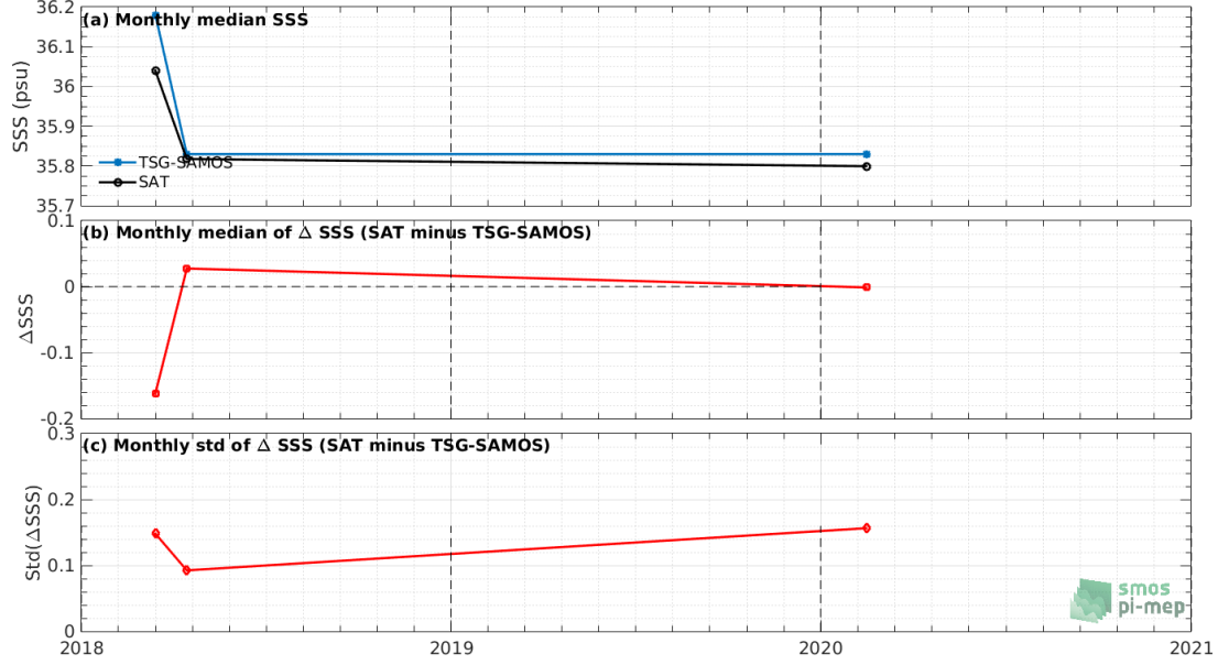
Figure 7: Time series of the monthly median SSS (top), median of \Delta\text{SSS} (Satellite - TSG-SAMOS) and Std of \Delta\text{SSS} (Satellite - TSG-SAMOS) over the South Atlantic Ocean Pi-MEP region considering all match-ups collected by the Pi-MEP.
