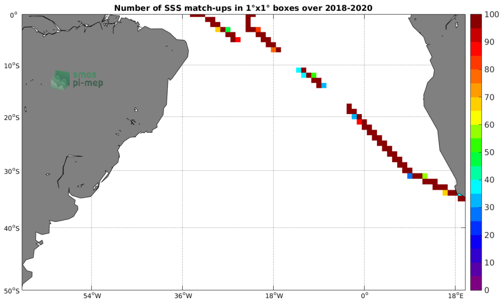
Figure 4: Number of SSS match-ups between TSG-SAMOS SSS and the SMAP-L3-RSS-V4-MONTHLY SSS product for the South Atlantic Ocean Pi-MEP region over 1^\circ \times 1^\circ boxes and for the full satellite product period.
