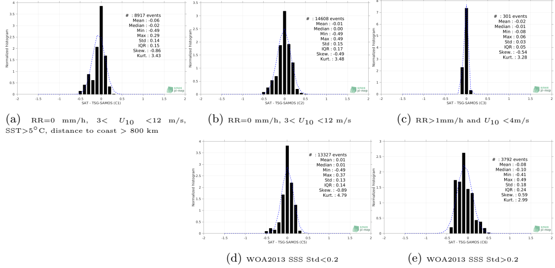
Figure 13: Normalized histogram of \Delta SSS (SMAP-L3-RSS-V4-MONTHLY - TSG-SAMOS) for 5 different subdatasets corresponding to: RR=0 mm/h, 3 < U_{10} < 12 m/s, SST>5°C, distance to coast > 800 km (a), RR=0 mm/h, 3 < U_{10} < 12 m/s (b), RR>1mm/h and U_{10} < 4 m/s (c), WOA2013 SSS Std<0.2 (d), WOA2013 SSS Std>0.2 (e).
