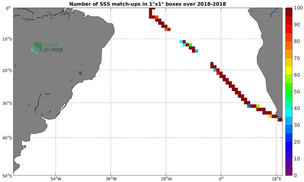
Figure 4: Number of SSS match-ups between TSG-SAMOS SSS and the SMAP-L3-RSS-V4-MONTHLY SSS product for the South Atlantic Ocean Pi-MEP region over 1°x1° boxes and for the full satellite product period.
