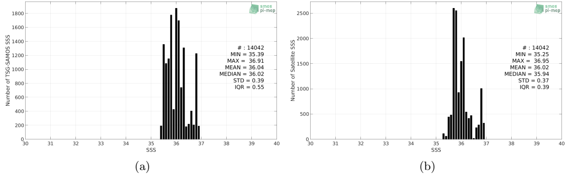
Figure 2: Histograms of SSS from TSG-SAMOS (a) and SMAP-L3-RSS-V4-MONTHLY (b) considering all match-up pairs per bins of 0.1 over the South Atlantic Ocean Pi-MEP region and for the full satellite product period.
