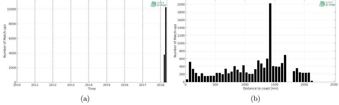
Figure 1: Number of match-ups between TSG-SAMOS and SMAP-L3-RSS-V4-MONTHLY SSS as a function of time (a) and as function of the distance to coast (b) over the South Atlantic Ocean Pi-MEP region and for the full satellite product period.
