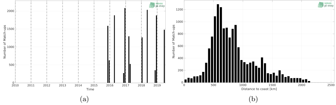
Figure 1: Number of match-ups between TSG (Polarstern) and SMAP SSS L3 v4 - Monthly (RSS) SSS as a function of time (a) and as function of the distance to coast (b) over the South Atlantic Ocean Pi-MEP region and for the full satellite product period.
