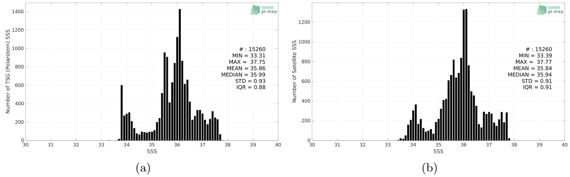
Figure 2: Histograms of SSS from TSG (Polarstern) (a) and SMAP SSS L3 v4 - Monthly (RSS) (b) considering all match-up pairs per bins of 0.1 over the South Atlantic Ocean Pi-MEP region and for the full satellite product period.
