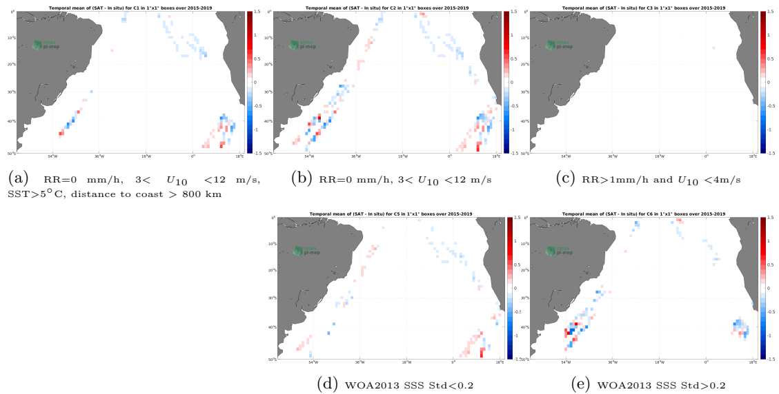
Figure 12: Temporal mean gridded over spatial boxes of size 1^\circ \times 1^\circ of \Delta SSS (SMAP SSS L3 v4 - Monthly (RSS) - TSG (Polarstern)) for 5 different subdatasets corresponding to:RR=0 mm/h, 3 < U_{10} < 12 m/s, SST >5^\circ\text{C} , distance to coast > 800 km (a), RR=0 mm/h, 3 < U_{10} < 12 m/s (b), RR >1 mm/h and U_{10} < 4 m/s (c), WOA2013 SSS Std <0.2 (d), WOA2013 SSS Std >0.2 (e).
