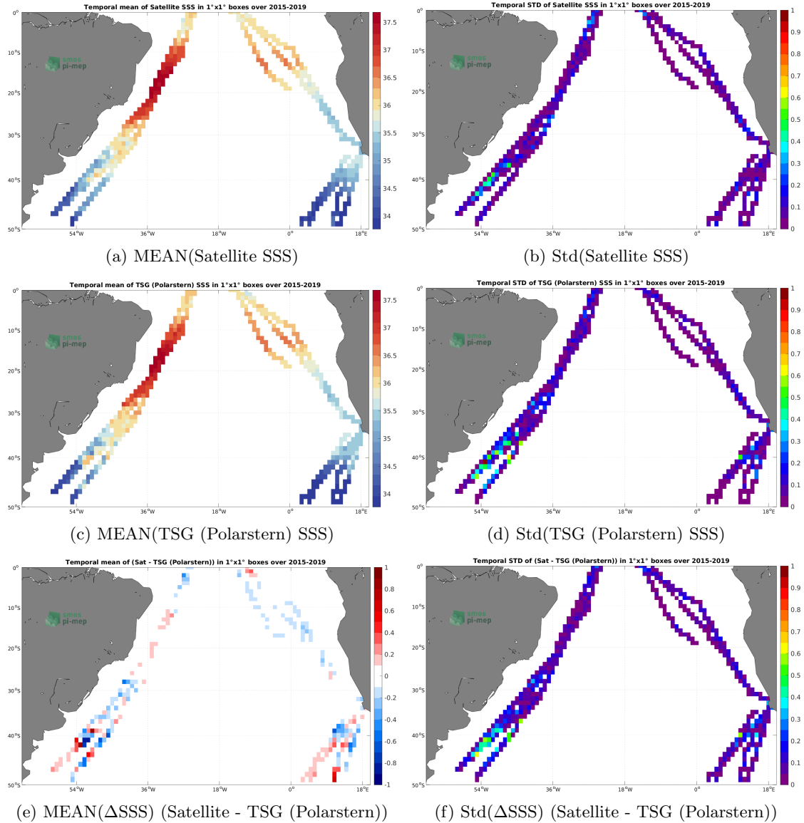
Figure 6: Temporal mean (left) and Std (right) of SSS from SMAP SSS L3 v4 - Monthly (RSS) (top), TSG (Polarstern) (middle), and of \Delta SSS (Satellite - TSG (Polarstern)). Only match-up pairs are used to generate these maps.
