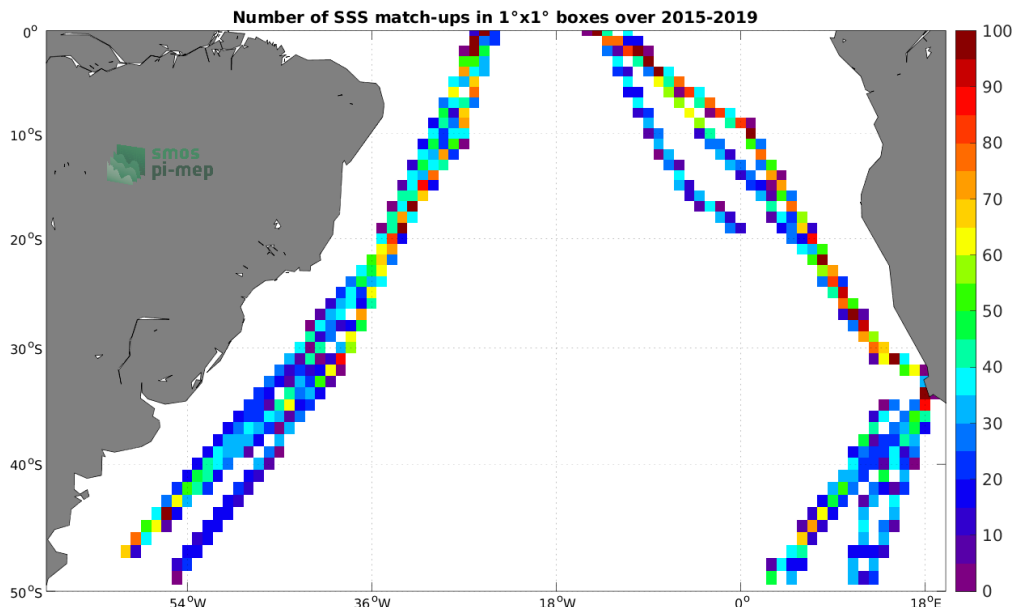
Figure 4: Number of SSS match-ups between TSG (Polarstern) SSS and the SMAP SSS L3 v4 - Monthly (RSS) SSS product for the South Atlantic Ocean Pi-MEP region over 1^\circ \times 1^\circ boxes and for the full satellite product period.
