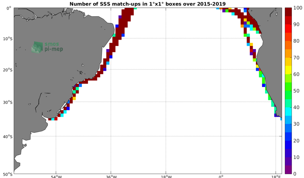
Figure 4: Number of SSS match-ups between TSG (LEGOS-DM) SSS and the SMAP SSS L3 v4 - Monthly (RSS) SSS product for the South Atlantic Ocean Pi-MEP region over 1^\circ \times 1^\circ boxes and for the full satellite product period.
