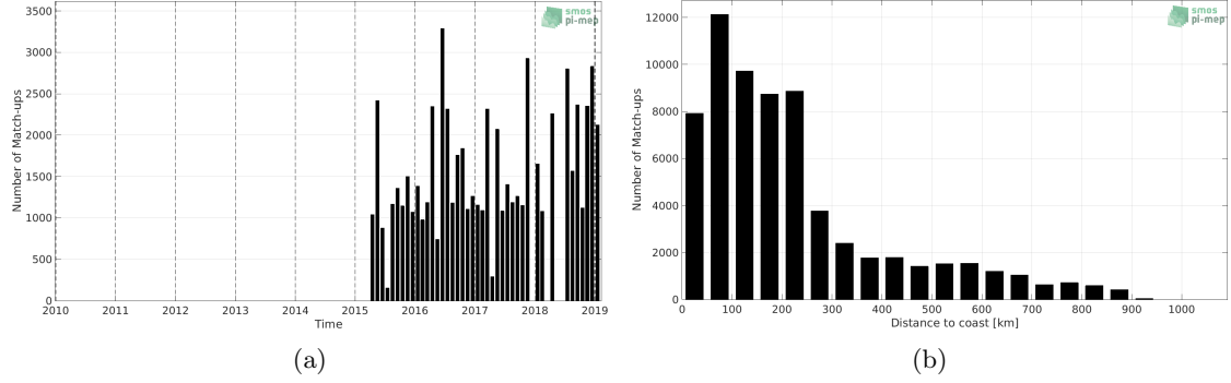
Figure 1: Number of match-ups between TSG (LEGOS-DM) and SMAP SSS L3 v4 - Monthly (RSS) SSS as a function of time (a) and as function of the distance to coast (b) over the South Atlantic Ocean Pi-MEP region and for the full satellite product period.
