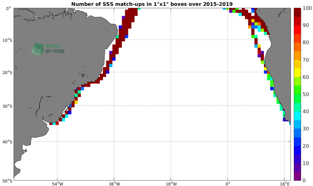
Figure 4: Number of SSS match-ups between TSG-LEGOS-DM SSS and the SMAP-L3-RSS-V4-MONTHLY SSS product for the South Atlantic Ocean Pi-MEP region over 1°x1° boxes and for the full satellite product period.
