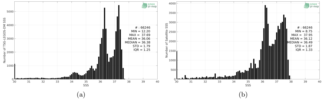
Figure 2: Histograms of SSS from TSG-LEGOS-DM (a) and SMAP-L3-RSS-V4-MONTHLY (b) considering all match-up pairs per bins of 0.1 over the South Atlantic Ocean Pi-MEP region and for the full satellite product period.
