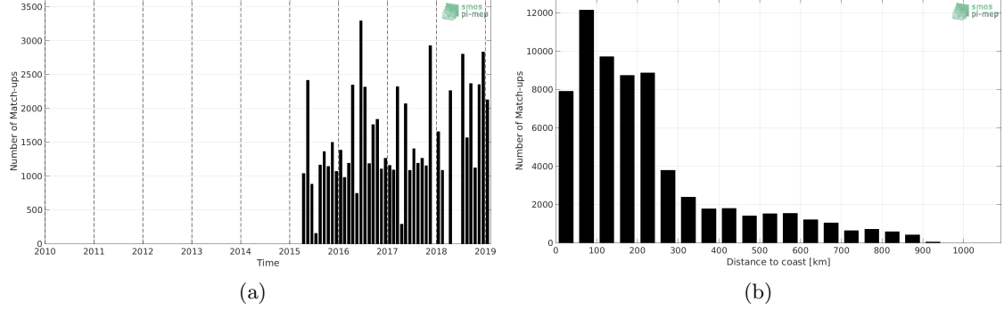
Figure 1: Number of match-ups between TSG-LEGOS-DM and SMAP-L3-RSS-V4-MONTHLY SSS as a function of time (a) and as function of the distance to coast (b) over the South Atlantic Ocean Pi-MEP region and for the full satellite product period.
