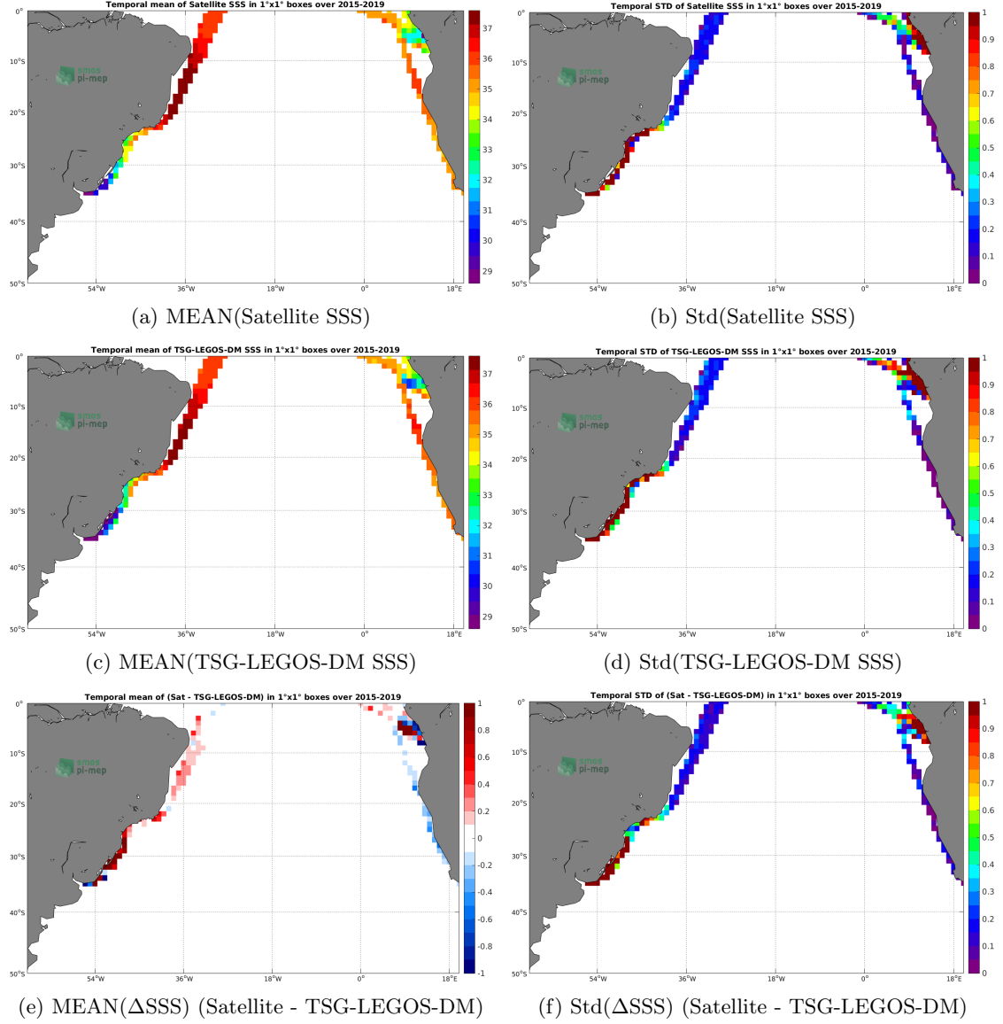
Figure 6: Temporal mean (left) and Std (right) of SSS from SMAP-L3-RSS-V4-MONTHLY (top), TSG-LEGOS-DM (middle), and of \Delta SSS (Satellite - TSG-LEGOS-DM). Only match-up pairs are used to generate these maps.
