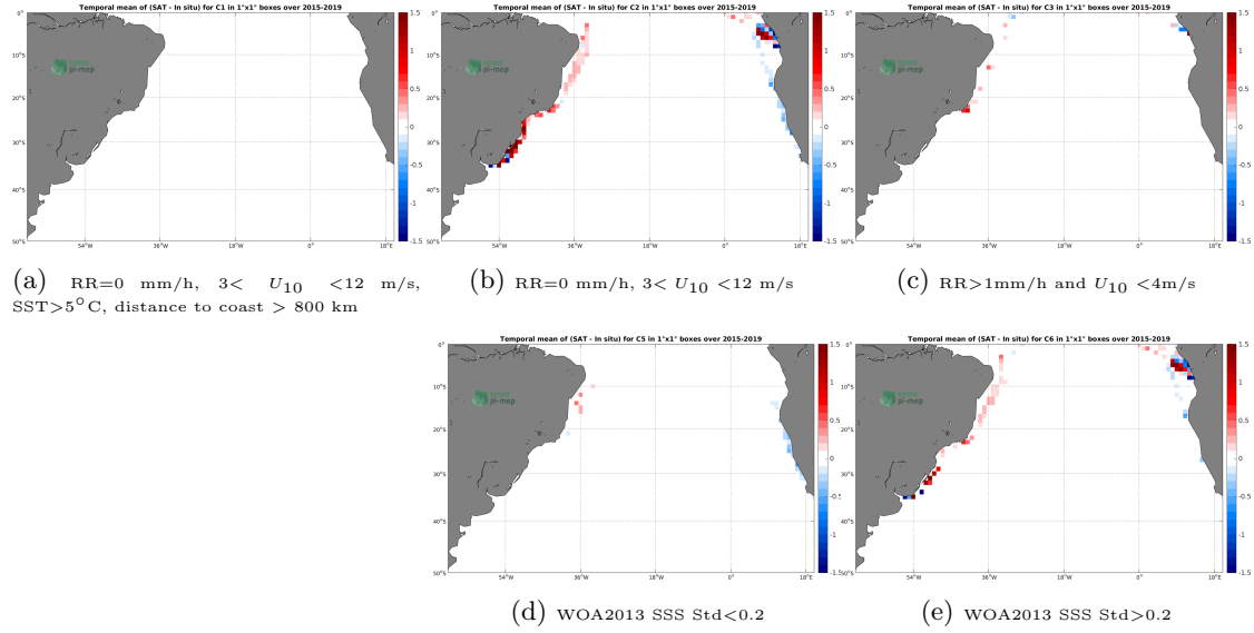
Figure 12: Temporal mean gridded over spatial boxes of size 1^\circ \times 1^\circ of \Delta SSS (SMAP-L3-RSS-V4-MONTHLY - TSG-LEGOS-DM) for 5 different subdatasets corresponding to: RR=0 mm/h, 3 < U_{10} < 12 m/s, SST > 5^\circ C , distance to coast > 800 km (a), RR=0 mm/h, 3 < U_{10} < 12 m/s (b), RR > 1 mm/h and U_{10} < 4 m/s (c), WOA2013 SSS Std < 0.2 (d), WOA2013 SSS Std > 0.2 (e).
