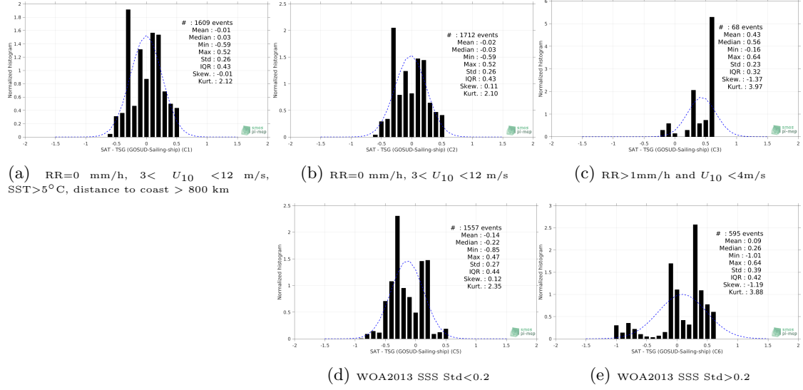
Figure 13: Normalized histogram of \Delta\text{SSS} (SMAP SSS L3 v4 - Monthly (RSS) - TSG (GOSUD-Sailing-ship)) for 5 different subdatasets corresponding to: RR=0 mm/h, 3 < U_{10} < 12 m/s, SST > 5^\circ\text{C} , distance to coast > 800 km (a), RR=0 mm/h, 3 < U_{10} < 12 m/s (b), RR > 1\text{mm/h} and U_{10} < 4\text{m/s} (c), WOA2013 SSS Std < 0.2 (d), WOA2013 SSS Std > 0.2 (e).
