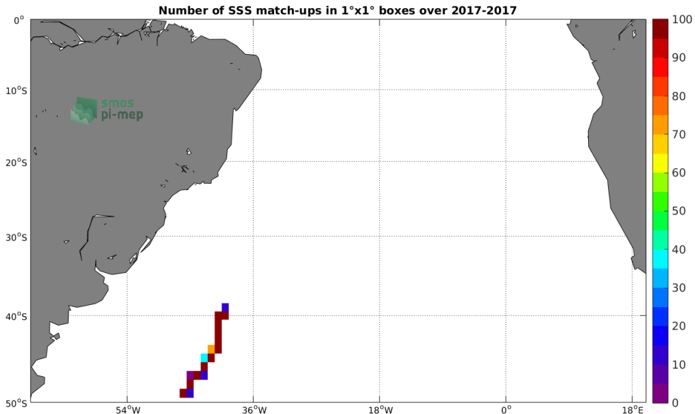
Figure 4: Number of SSS match-ups between TSG (GOSUD-Sailing-ship) SSS and the SMAP SSS L3 v4 - Monthly (RSS) SSS product for the South Atlantic Ocean Pi-MEP region over 1^\circ \times 1^\circ boxes and for the full satellite product period.
