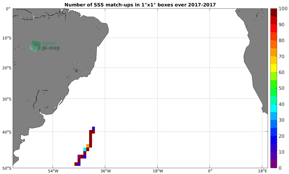
Figure 4: Number of SSS match-ups between TSG (GOSUD-Sailing-ship) SSS and the SMAP SSS L3 v4 - Monthly (RSS) SSS product for the South Atlantic Ocean Pi-MEP region over 1°x1° boxes and for the full satellite product period.
