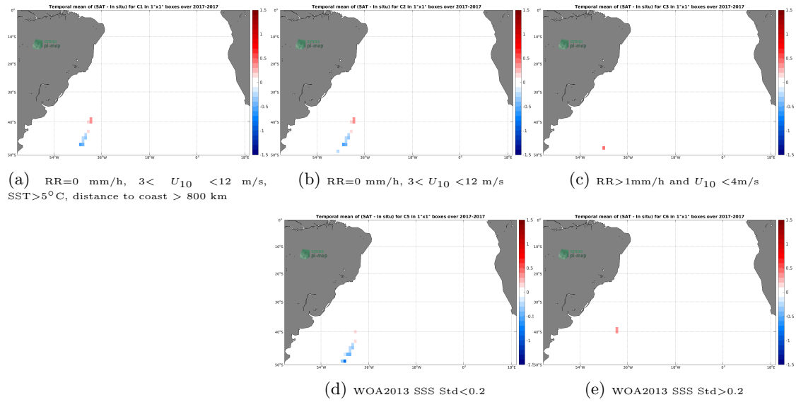
Figure 12: Temporal mean gridded over spatial boxes of size 1^\circ \times 1^\circ of \Delta SSS (SMAP SSS L3 v4 - Monthly (RSS) - TSG (GOSUD-Sailing-ship)) for 5 different subdatasets corresponding to: RR=0 mm/h, 3 < U_{10} < 12 m/s, SST > 5^\circ\text{C} , distance to coast > 800 km (a), RR=0 mm/h, 3 < U_{10} < 12 m/s (b), RR > 1\text{mm/h} and U_{10} < 4\text{m/s} (c), WOA2013 SSS Std < 0.2 (d), WOA2013 SSS Std > 0.2 (e).
