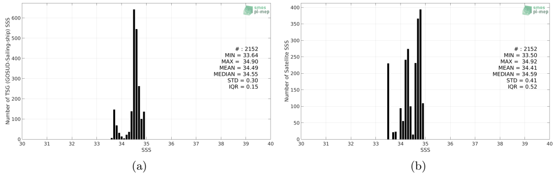
Figure 2: Histograms of SSS from TSG (GOSUD-Sailing-ship) (a) and SMAP SSS L3 v4 - Monthly (RSS) (b) considering all match-up pairs per bins of 0.1 over the South Atlantic Ocean Pi-MEP region and for the full satellite product period.
