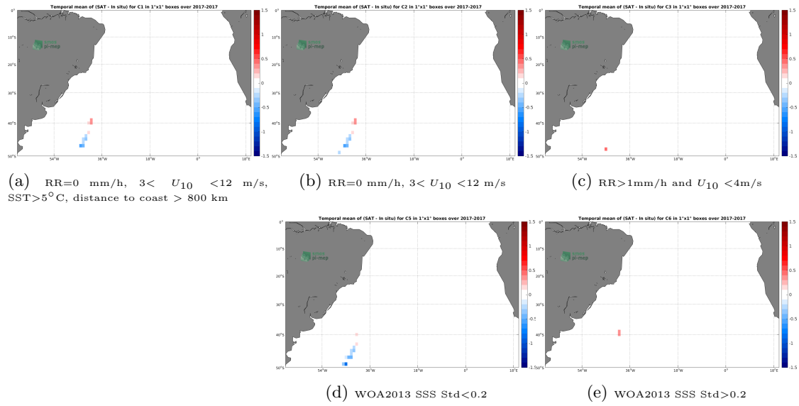
Figure 12: Temporal mean gridded over spatial boxes of size 1^\circ \times 1^\circ of \Delta SSS (SMAP-L3-RSS-V4-MONTHLY - TSG-GOSUD-Sailing-ship) for 5 different subdatasets corresponding to: RR=0 mm/h, 3 < U_{10} < 12 m/s, SST > 5^\circ C , distance to coast > 800 km (a), RR=0 mm/h, 3 < U_{10} < 12 m/s (b), RR > 1 mm/h and U_{10} < 4 m/s (c), WOA2013 SSS Std < 0.2 (d), WOA2013 SSS Std > 0.2 (e).
