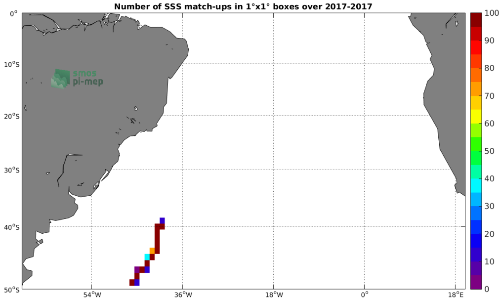
Figure 4: Number of SSS match-ups between TSG-GOSUD-Sailing-ship SSS and the SMAP-L3-RSS-V4-MONTHLY SSS product for the South Atlantic Ocean Pi-MEP region over 1°x1° boxes and for the full satellite product period.
