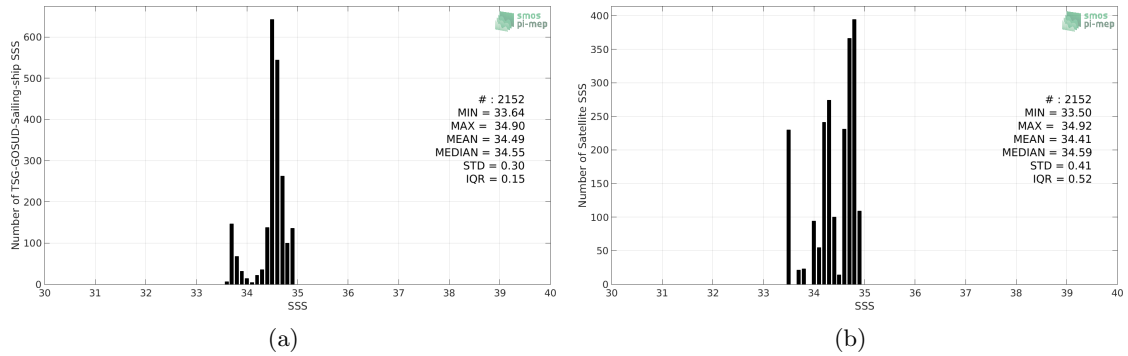
Figure 2: Histograms of SSS from TSG-GOSUD-Sailing-ship (a) and SMAP-L3-RSS-V4-MONTHLY (b) considering all match-up pairs per bins of 0.1 over the South Atlantic Ocean Pi-MEP region and for the full satellite product period.
