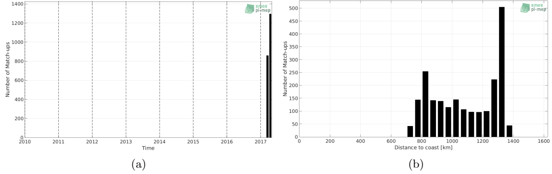
Figure 1: Number of match-ups between TSG-GOSUD-Sailing-ship and SMAP-L3-RSS-V4-MONTHLY SSS as a function of time (a) and as function of the distance to coast (b) over the South Atlantic Ocean Pi-MEP region and for the full satellite product period.
