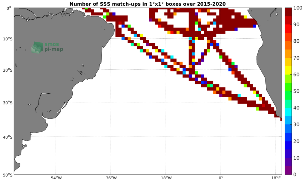
Figure 4: Number of SSS match-ups between TSG (GOSUD-Research-vessel) SSS and the SMAP SSS L3 v4 - Monthly (RSS) SSS product for the South Atlantic Ocean Pi-MEP region over 1^\circ \times 1^\circ boxes and for the full satellite product period.
