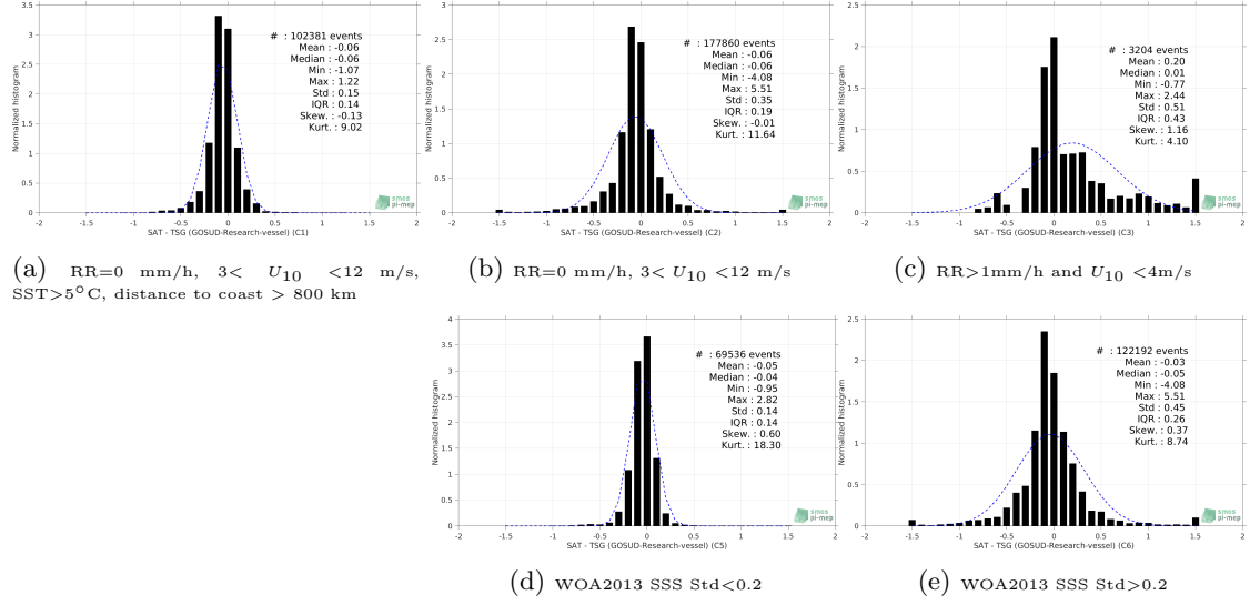
Figure 13: Normalized histogram of \Delta SSS (SMAP SSS L3 v4 - Monthly (RSS) - TSG (GOSUD-Research-vessel)) for 5 different subdatasets corresponding to: RR=0 mm/h, 3 < U_{10} < 12 m/s, SST>5°C, distance to coast > 800 km (a), RR=0 mm/h, 3 < U_{10} < 12 m/s (b), RR>1mm/h and U_{10} < 4 m/s (c), WOA2013 SSS Std<0.2 (d), WOA2013 SSS Std>0.2 (e).
