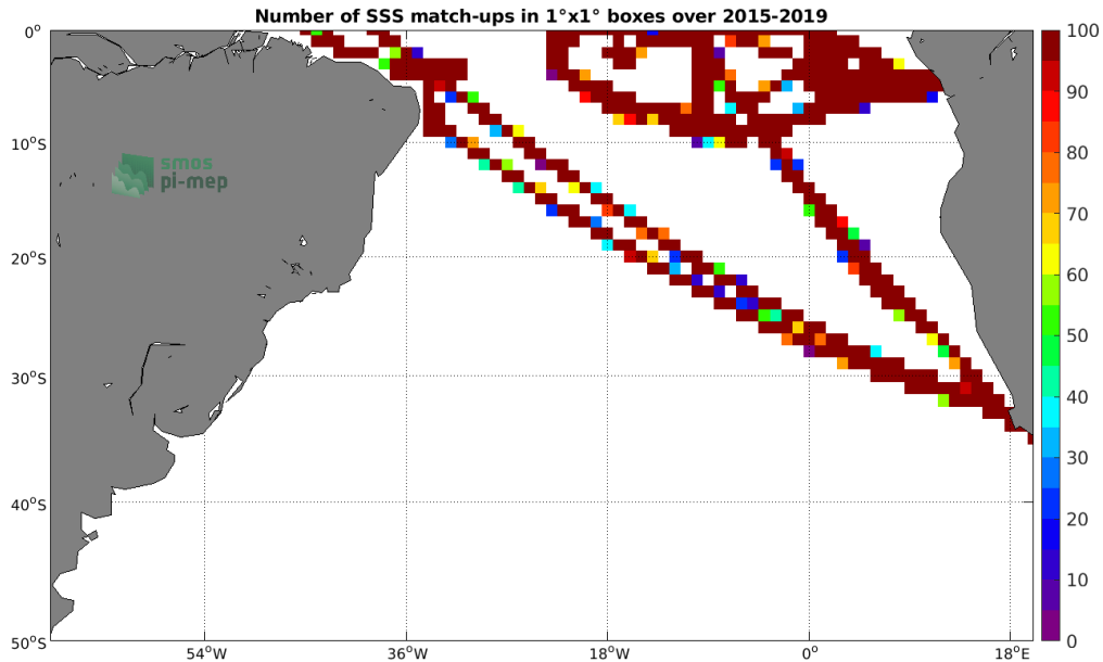
Figure 4: Number of SSS match-ups between TSG (GOSUD-Research-vessel) SSS and the SMAP SSS L3 v4 - Monthly (RSS) SSS product for the South Atlantic Ocean Pi-MEP region over 1^\circ \times 1^\circ boxes and for the full satellite product period.
