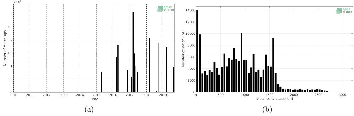
Figure 1: Number of match-ups between TSG (GOSUD-Research-vessel) and SMAP SSS L3 v4 - Monthly (RSS) SSS as a function of time (a) and as function of the distance to coast (b) over the South Atlantic Ocean Pi-MEP region and for the full satellite product period.
