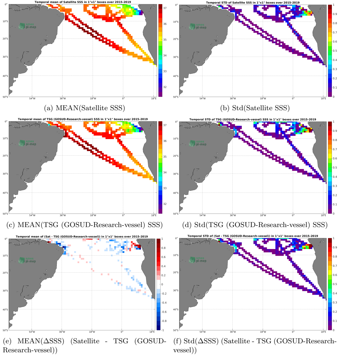
Figure 6: Temporal mean (left) and Std (right) of SSS from SMAP SSS L3 v4 - Monthly (RSS) (top), TSG (GOSUD-Research-vessel) (middle), and of \Delta SSS (Satellite - TSG (GOSUD-Research-vessel)). Only match-up pairs are used to generate these maps.
