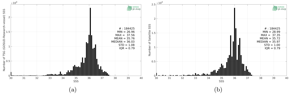
Figure 2: Histograms of SSS from TSG (GOSUD-Research-vessel) (a) and SMAP SSS L3 v4 - Monthly (RSS) (b) considering all match-up pairs per bins of 0.1 over the South Atlantic Ocean Pi-MEP region and for the full satellite product period.
