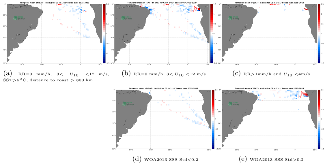
Figure 12: Temporal mean gridded over spatial boxes of size 1^\circ \times 1^\circ of \Delta SSS (SMAP SSS L3 v4 - Monthly (RSS) - TSG (GOSUD-Research-vessel)) for 5 different subdatasets corresponding to: RR=0 mm/h, 3 < U_{10} < 12 m/s, SST > 5^\circ C , distance to coast > 800 km (a), RR=0 mm/h, 3 < U_{10} < 12 m/s (b), RR > 1 mm/h and U_{10} < 4 m/s (c), WOA2013 SSS Std < 0.2 (d), WOA2013 SSS Std > 0.2 (e).
