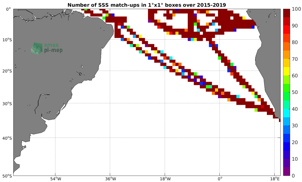
Figure 4: Number of SSS match-ups between TSG (GOSUD-Research-vessel) SSS and the SMAP SSS L3 v4 - Monthly (RSS) SSS product for the South Atlantic Ocean Pi-MEP region over 1°x1° boxes and for the full satellite product period.
