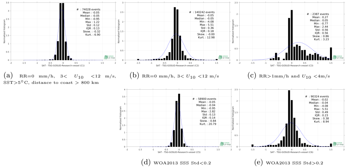
Figure 13: Normalized histogram of \Delta SSS (SMAP-L3-RSS-V4-MONTHLY - TSG-GOSUD-Research-vessel) for 5 different subdatasets corresponding to: RR=0 mm/h, 3 < U_{10} < 12 m/s, SST > 5°C, distance to coast > 800 km (a), RR=0 mm/h, 3 < U_{10} < 12 m/s (b), RR > 1mm/h and U_{10} < 4 m/s (c), WOA2013 SSS Std < 0.2 (d), WOA2013 SSS Std > 0.2 (e).
