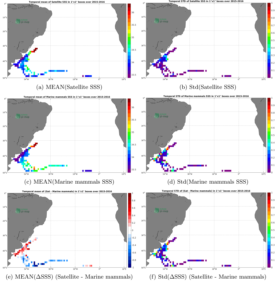
Figure 6: Temporal mean (left) and Std (right) of SSS from SMAP SSS L3 v4 - Monthly (RSS) (top), Marine mammals (middle), and of \Delta SSS (Satellite - Marine mammals). Only match-up pairs are used to generate these maps.
