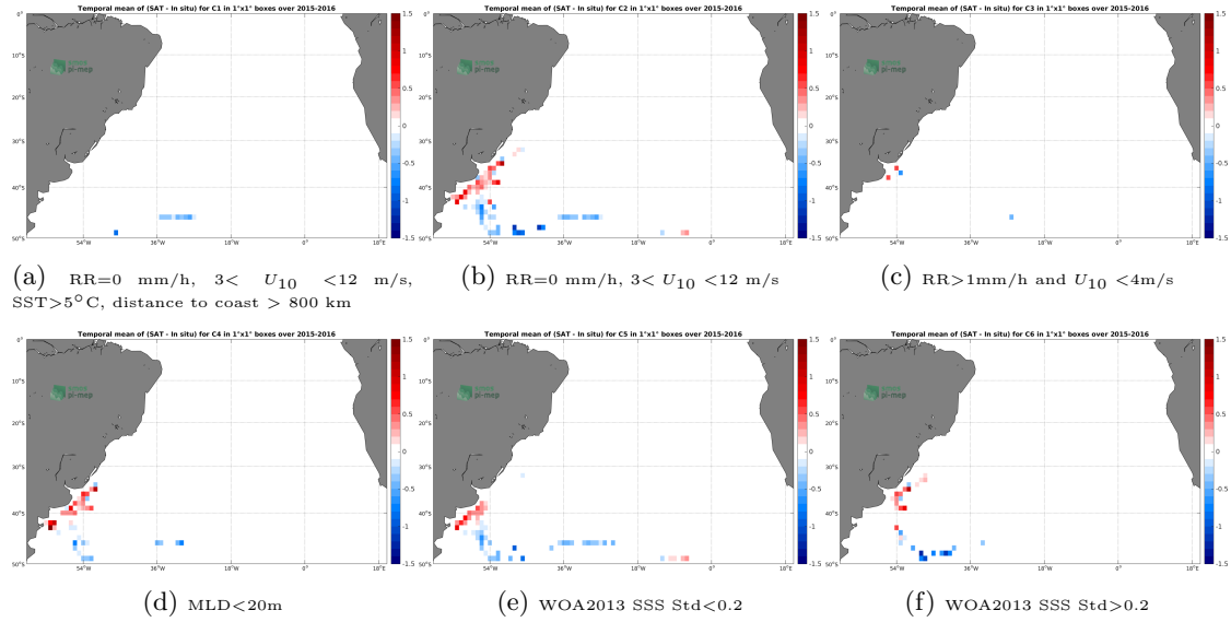
Figure 12: Temporal mean gridded over spatial boxes of size 1^\circ \times 1^\circ of \Delta SSS (SMAP SSS L3 v4 - Monthly (RSS) - Marine mammals) for 6 different subdatasets corresponding to: RR=0 mm/h, 3 < U_{10} < 12 m/s, SST > 5^\circ\text{C} , distance to coast > 800 km (a), RR=0 mm/h, 3 < U_{10} < 12 m/s (b), RR > 1 mm/h and U_{10} < 4 m/s (c), MLD < 20 m (d), WOA2013 SSS Std < 0.2 (e), WOA2013 SSS Std > 0.2 (f).
