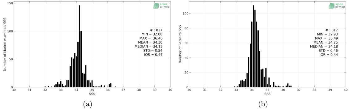
Figure 2: Histograms of SSS from Marine mammals (a) and SMAP SSS L3 v4 - Monthly (RSS) (b) considering all match-up pairs per bins of 0.1 over the South Atlantic Ocean Pi-MEP region and for the full satellite product period.
