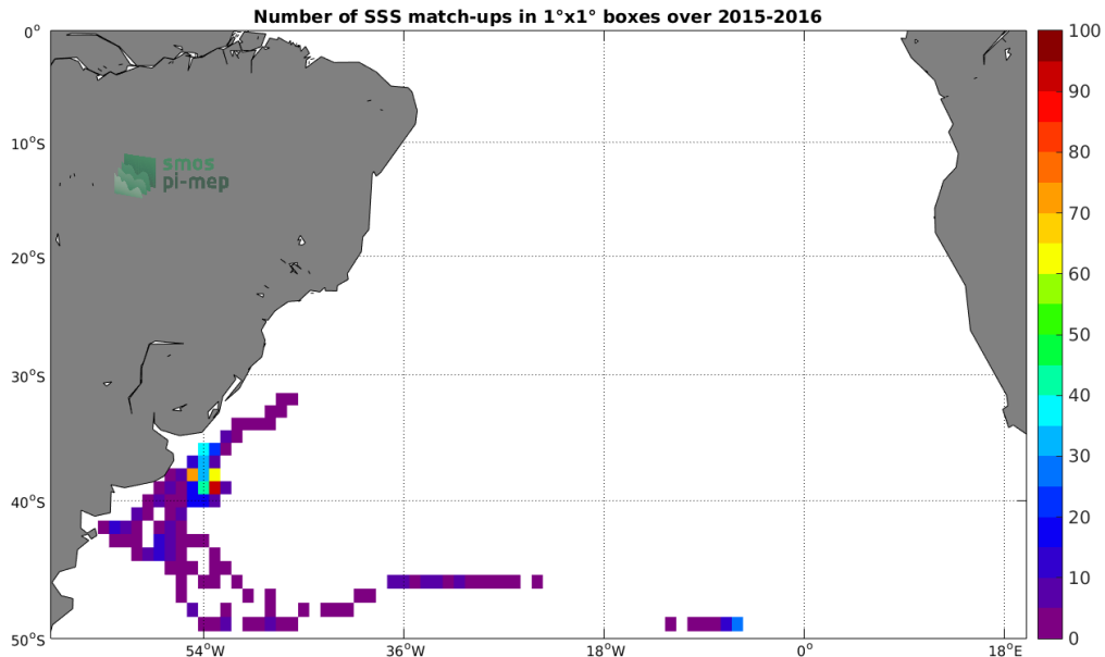
Figure 4: Number of SSS match-ups between Marine mammals SSS and the SMAP SSS L3 v4 - Monthly (RSS) SSS product for the South Atlantic Ocean Pi-MEP region over 1^\circ \times 1^\circ boxes and for the full satellite product period.
