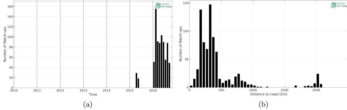
Figure 1: Number of match-ups between Marine mammals and SMAP SSS L3 v4 - Monthly (RSS) SSS as a function of time (a) and as function of the distance to coast (b) over the South Atlantic Ocean Pi-MEP region and for the full satellite product period.
