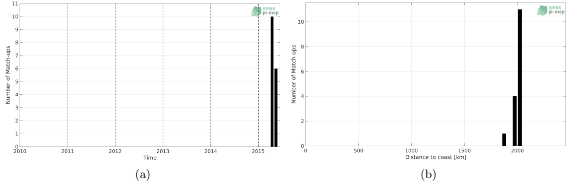
Figure 1: Number of match-ups between Sea mammals and SMAP SSS L3 v4 - Monthly (RSS) SSS as a function of time (a) and as function of the distance to coast (b) over the South Atlantic Ocean Pi-MEP region and for the full satellite product period.
