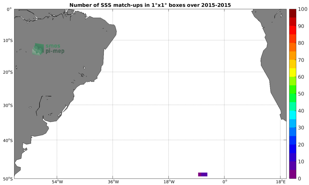
Figure 4: Number of SSS match-ups between Sea mammals SSS and the SMAP SSS L3 v4 - Monthly (RSS) SSS product for the South Atlantic Ocean Pi-MEP region over 1°x1° boxes and for the full satellite product period.
