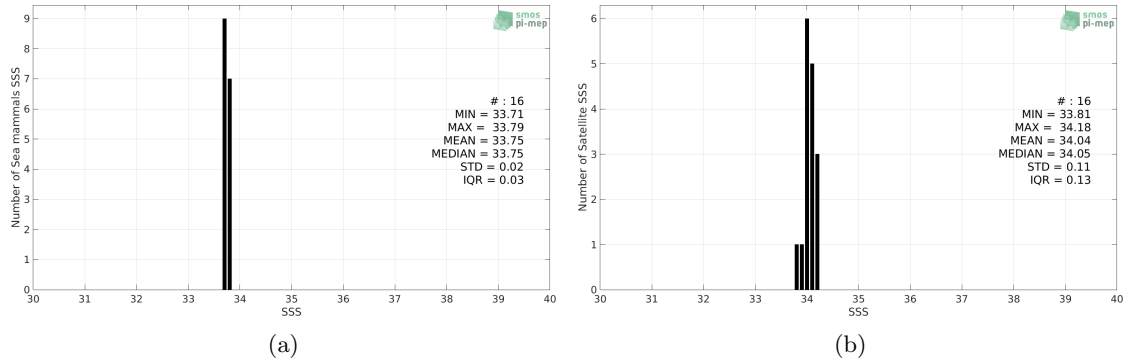
Figure 2: Histograms of SSS from Sea mammals (a) and SMAP SSS L3 v4 - Monthly (RSS) (b) considering all match-up pairs per bins of 0.1 over the South Atlantic Ocean Pi-MEP region and for the full satellite product period.
