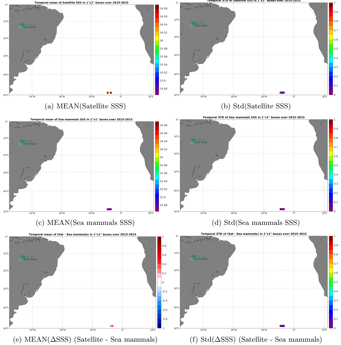
Figure 6: Temporal mean (left) and Std (right) of SSS from SMAP SSS L3 v4 - Monthly (RSS) (top), Sea mammals (middle), and of \Delta SSS (Satellite - Sea mammals). Only match-up pairs are used to generate these maps.
