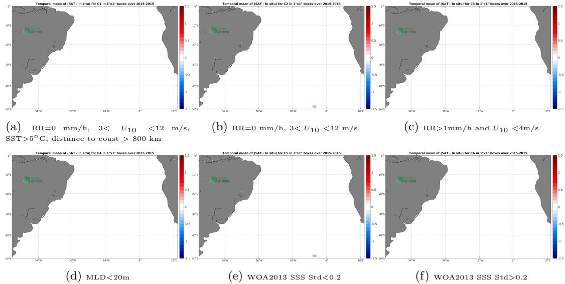
Figure 12: Temporal mean gridded over spatial boxes of size 1^{\circ}\times 1^{\circ} of \Delta\text{SSS} (SMAP-L3-RSS-V4-MONTHLY - Sea mammals) for 6 different subdatasets corresponding to:RR=0 mm/h, 3 < U_{10} < 12 m/s, SST >5^{\circ}\text{C} , distance to coast > 800 km (a), RR=0 mm/h, 3 < U_{10} < 12 m/s (b), RR >1\text{mm/h} and U_{10} < 4\text{m/s} (c),MLD <20\text{m} (d),WOA2013 SSS Std <0.2 (e),WOA2013 SSS Std >0.2 (f).
