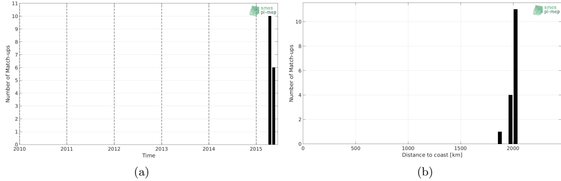
Figure 1: Number of match-ups between Sea mammals and SMAP-L3-RSS-V4-MONTHLY SSS as a function of time (a) and as function of the distance to coast (b) over the South Atlantic Ocean Pi-MEP region and for the full satellite product period.
