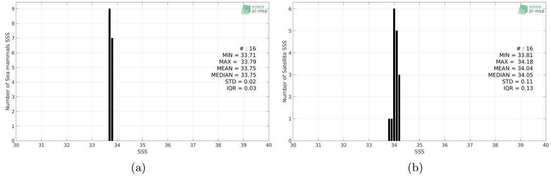
Figure 2: Histograms of SSS from Sea mammals (a) and SMAP-L3-RSS-V4-MONTHLY (b) considering all match-up pairs per bins of 0.1 over the South Atlantic Ocean Pi-MEP region and for the full satellite product period.
