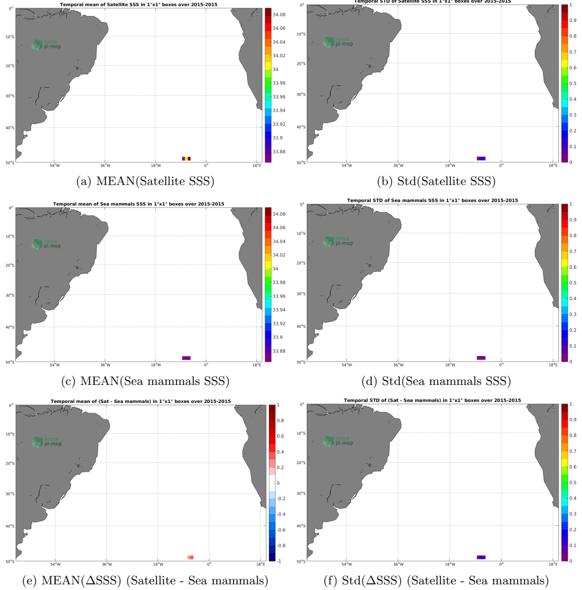
Figure 6: Temporal mean (left) and Std (right) of SSS from SMAP-L3-RSS-V4-MONTHLY (top), Sea mammals (middle), and of \Delta SSS (Satellite - Sea mammals). Only match-up pairs are used to generate these maps.
