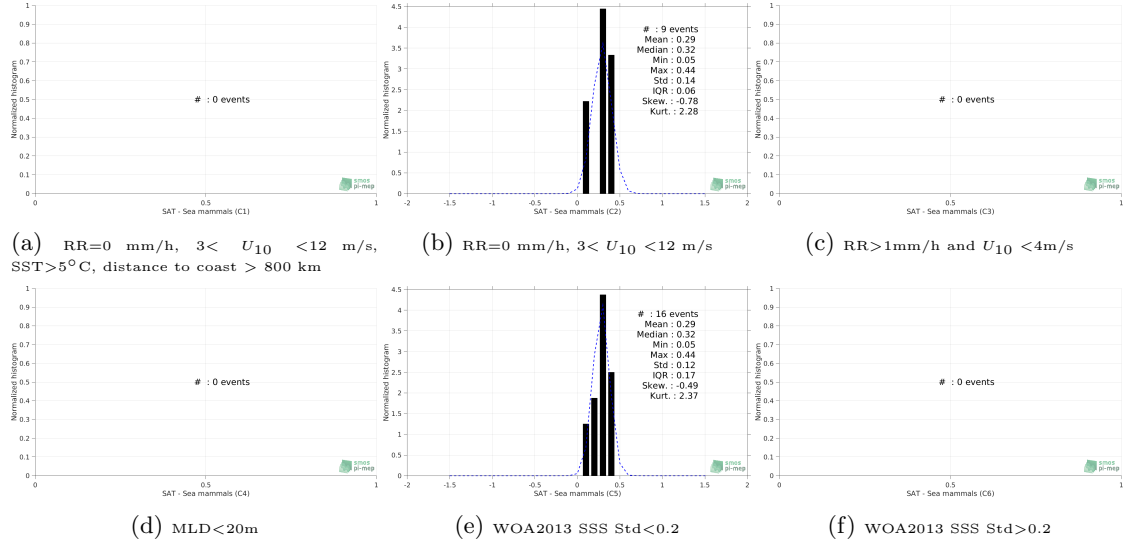
Figure 13: Normalized histogram of \Delta\text{SSS} (SMAP-L3-RSS-V4-MONTHLY - Sea mammals) for 6 different subdatasets corresponding to: RR=0 mm/h, 3 < U_{10} < 12 m/s, SST > 5^\circ\text{C} , distance to coast > 800 km (a), RR=0 mm/h, 3 < U_{10} < 12 m/s (b), RR > 1\text{mm/h} and U_{10} < 4\text{m/s} (c), MLD < 20\text{m} (d), WOA2013 SSS Std < 0.2 (e), WOA2013 SSS Std > 0.2 (f).
