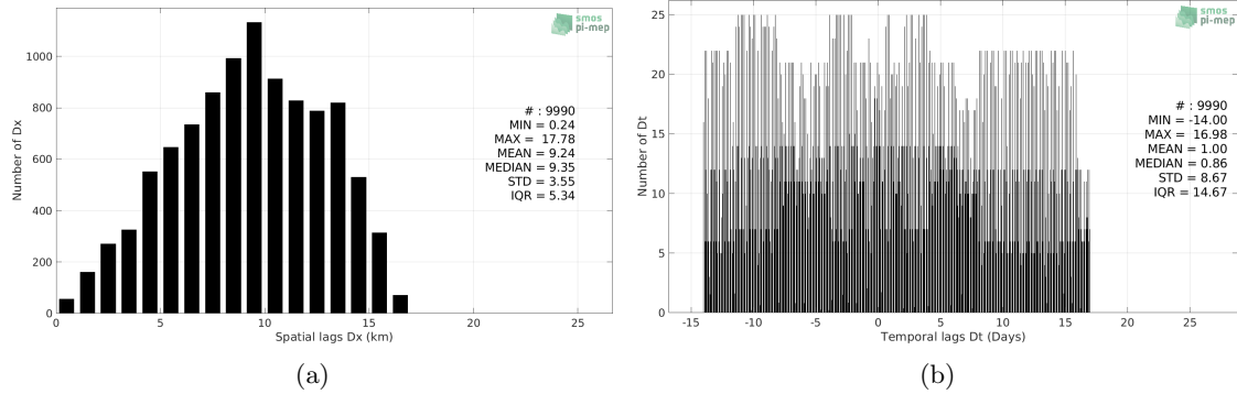
Figure 4: Histograms of the spatial (a) and temporal (b) lags between the location/time of the Surface drifters measurement and the date of the corresponding SMAP SSS L3 v4 - Monthly (RSS) SSS pixel.
