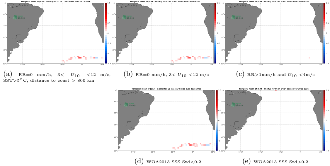
Figure 11: Temporal mean gridded over spatial boxes of size 1^{\circ}\times 1^{\circ} of \Delta\text{SSS} (SMAP SSS L3 v4 - Monthly (RSS) - Surface drifters) for 5 different subdatasets corresponding to:RR=0 mm/h, 3 < U_{10} < 12 m/s, SST >5^{\circ}\text{C} , distance to coast > 800 km (a), RR=0 mm/h, 3 < U_{10} < 12 m/s (b), RR >1 mm/h and U_{10} < 4 m/s (c), WOA2013 SSS Std <0.2 (d), WOA2013 SSS Std >0.2 (e).
