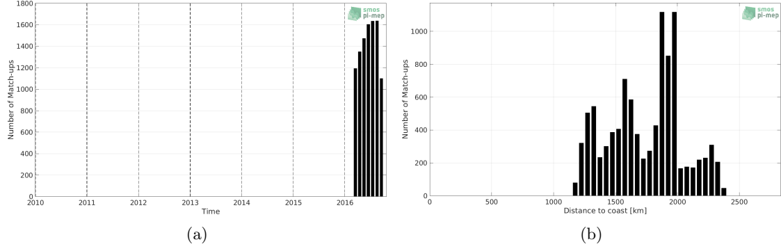
Figure 1: Number of match-ups between Surface drifters and SMAP SSS L3 v4 - Monthly (RSS) SSS as a function of time (a) and as function of the distance to coast (b) over the South Atlantic Ocean Pi-MEP region and for the full satellite product period.
