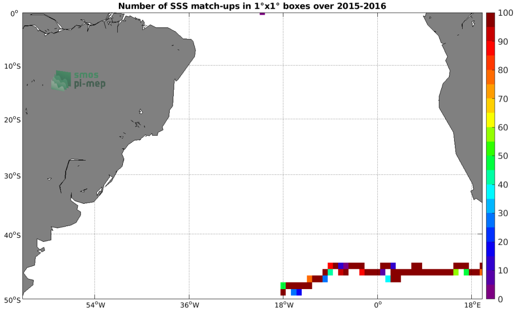
Figure 3: Number of SSS match-ups between Surface drifters SSS and the SMAP SSS L3 v4 - Monthly (RSS) SSS product for the South Atlantic Ocean Pi-MEP region over 1^\circ \times 1^\circ boxes and for the full satellite product period.
