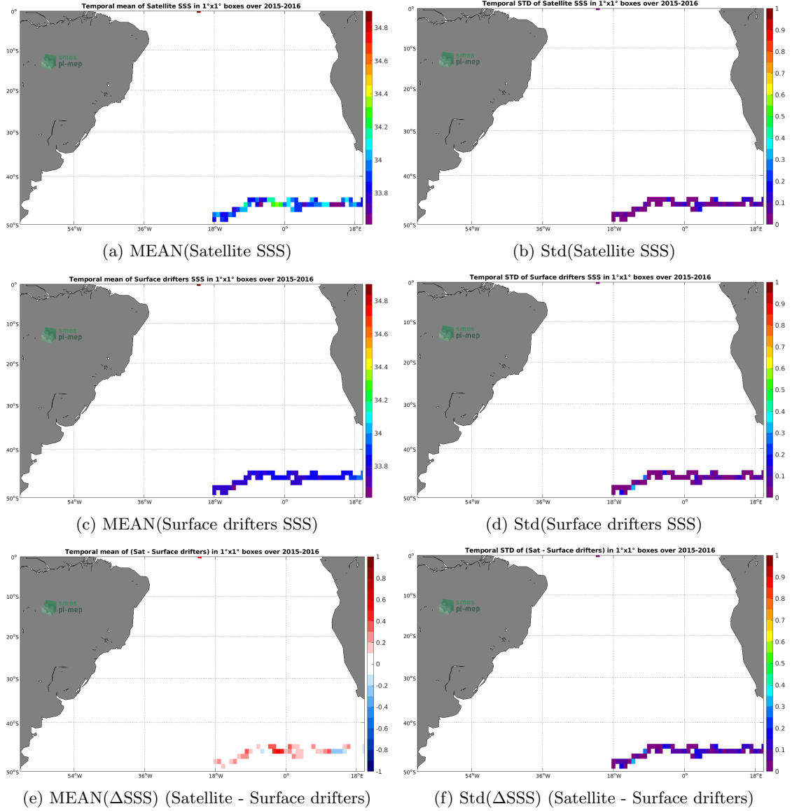
Figure 5: Temporal mean (left) and Std (right) of SSS from SMAP SSS L3 v4 - Monthly (RSS) (top), Surface drifters (middle), and of \Delta SSS (Satellite - Surface drifters). Only match-up pairs are used to generate these maps.
