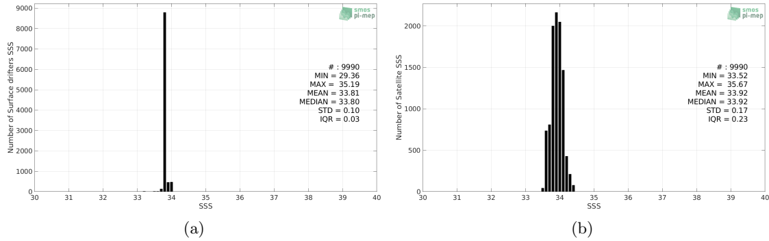
Figure 2: Histograms of SSS from Surface drifters (a) and SMAP SSS L3 v4 - Monthly (RSS) (b) considering all match-up pairs per bins of 0.1 over the South Atlantic Ocean Pi-MEP region and for the full satellite product period.
