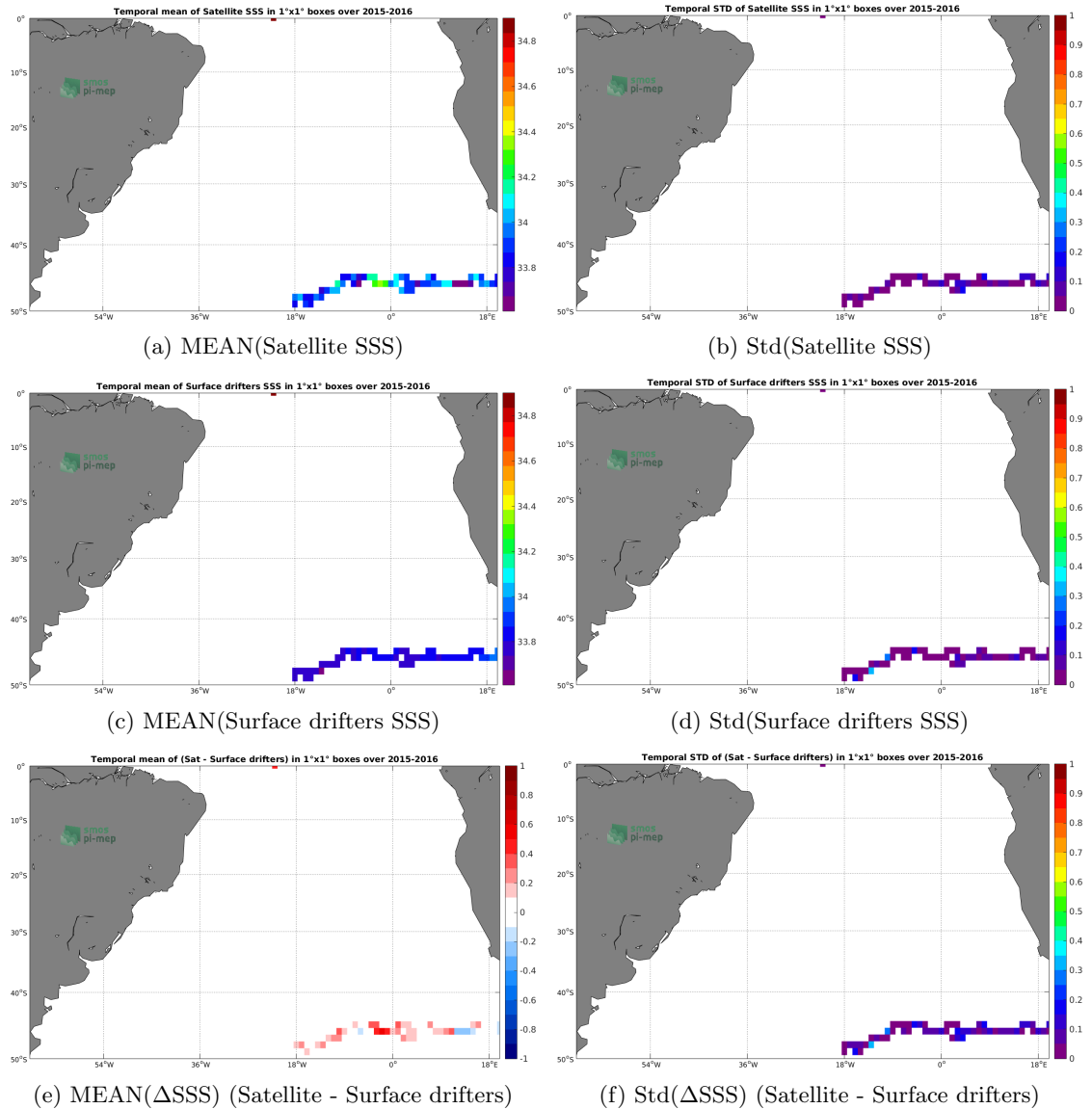
Figure 5: Temporal mean (left) and Std (right) of SSS from SMAP-L3-RSS-V4-MONTHLY (top), Surface drifters (middle), and of \Delta SSS (Satellite - Surface drifters). Only match-up pairs are used to generate these maps.
