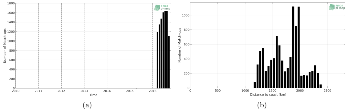
Figure 1: Number of match-ups between Surface drifters and SMAP-L3-RSS-V4-MONTHLY SSS as a function of time (a) and as function of the distance to coast (b) over the South Atlantic Ocean Pi-MEP region and for the full satellite product period.
