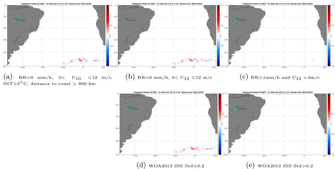
Figure 11: Temporal mean gridded over spatial boxes of size 1^{\circ}\times 1^{\circ} of \Delta\text{SSS} (SMAP-L3-RSS-V4-MONTHLY - Surface drifters) for 5 different subdatasets corresponding to:RR=0 mm/h, 3 < U_{10} < 12 m/s, SST > 5^{\circ}\text{C} , distance to coast > 800 km (a), RR=0 mm/h, 3 < U_{10} < 12 m/s (b), RR > 1 mm/h and U_{10} < 4 m/s (c), WOA2013 SSS Std < 0.2 (d), WOA2013 SSS Std > 0.2 (e).
