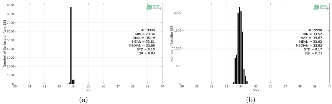
Figure 2: Histograms of SSS from Surface drifters (a) and SMAP-L3-RSS-V4-MONTHLY (b) considering all match-up pairs per bins of 0.1 over the South Atlantic Ocean Pi-MEP region and for the full satellite product period.
