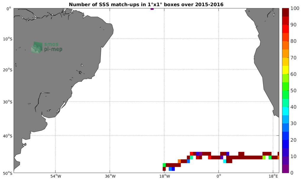
Figure 3: Number of SSS match-ups between Surface drifters SSS and the SMAP-L3-RSS-V4-MONTHLY SSS product for the South Atlantic Ocean Pi-MEP region over 1^\circ \times 1^\circ boxes and for the full satellite product period.
