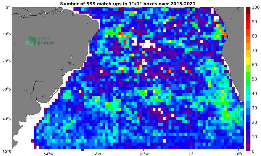
Figure 4: Number of SSS match-ups between Argo SSS and the SMAP SSS L3 v4 - Monthly (RSS) SSS product for the South Atlantic Ocean Pi-MEP region over 1°x1° boxes and for the full satellite product period.
