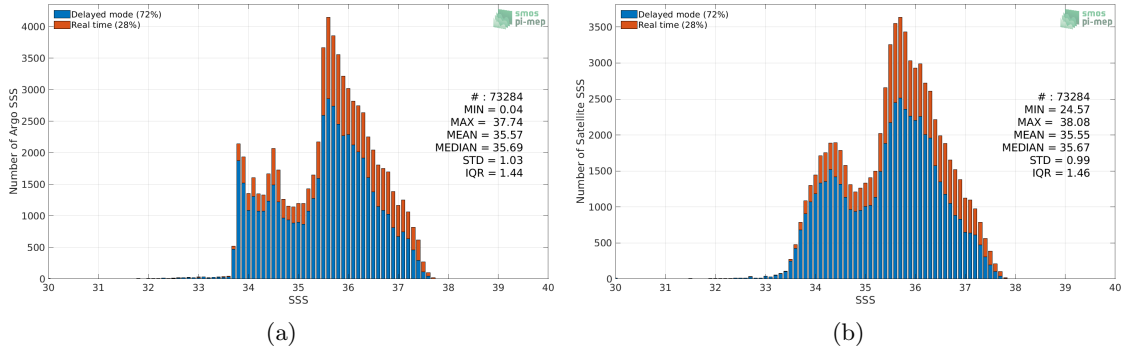
Figure 2: Histograms of SSS from Argo (a) and SMAP SSS L3 v4 - Monthly (RSS) (b) considering all match-up pairs per bins of 0.1 over the South Atlantic Ocean Pi-MEP region and for the full satellite product period.
