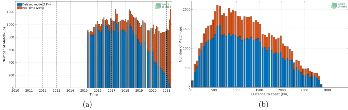
Figure 1: Number of match-ups between Argo and SMAP SSS L3 v4 - Monthly (RSS) SSS as a function of time (a) and as function of the distance to coast (b) over the South Atlantic Ocean Pi-MEP region and for the full satellite product period.
