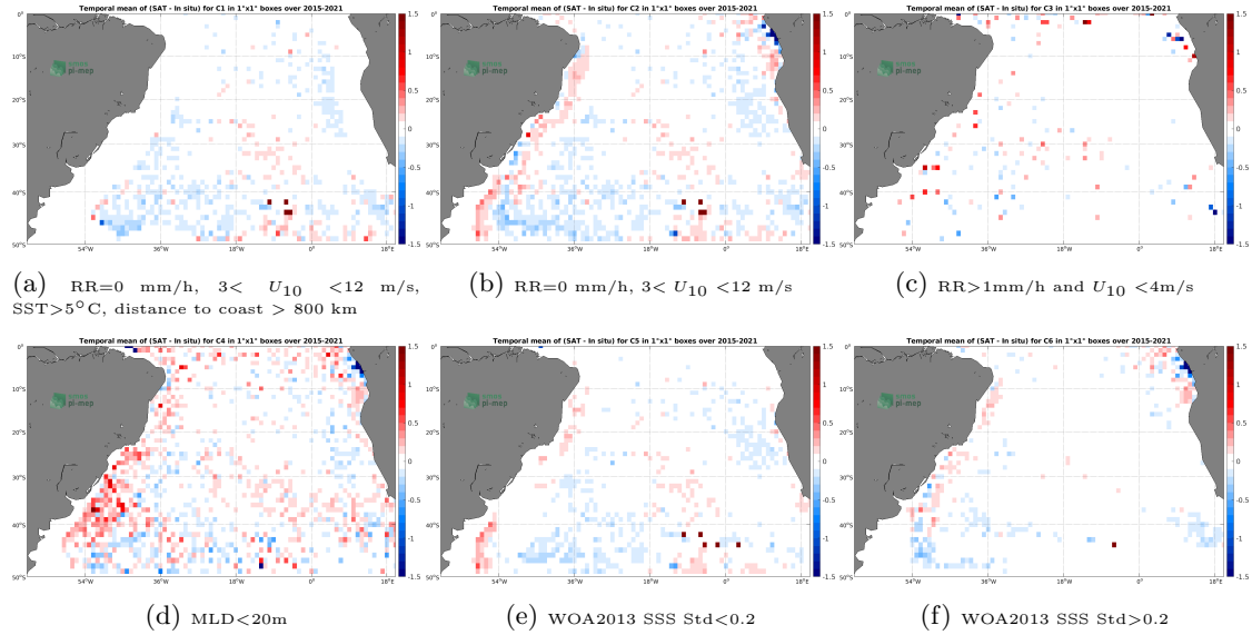
Figure 12: Temporal mean gridded over spatial boxes of size 1^\circ \times 1^\circ of \Delta SSS (SMAP SSS L3 v4 - Monthly (RSS) - Argo) for 6 different subdatasets corresponding to: RR=0 mm/h, 3 < U_{10} < 12 m/s, SST > 5^\circ\text{C} , distance to coast > 800 km (a), RR=0 mm/h, 3 < U_{10} < 12 m/s (b), RR > 1 mm/h and U_{10} < 4 m/s (c), MLD < 20 m (d), WOA2013 SSS Std < 0.2 (e), WOA2013 SSS Std > 0.2 (f).
