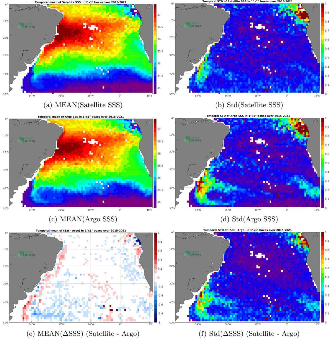
Figure 6: Temporal mean (left) and Std (right) of SSS from SMAP SSS L3 v4 - Monthly (RSS) (top), Argo (middle), and of \Delta SSS (Satellite - Argo). Only match-up pairs are used to generate these maps.
