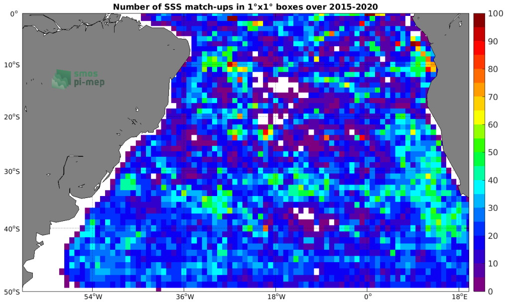
Figure 4: Number of SSS match-ups between Argos SSS and the SMAP SSS L3 v4 - Monthly (RSS) SSS product for the South Atlantic Ocean Pi-MEP region over 1°x1° boxes and for the full satellite product period.
