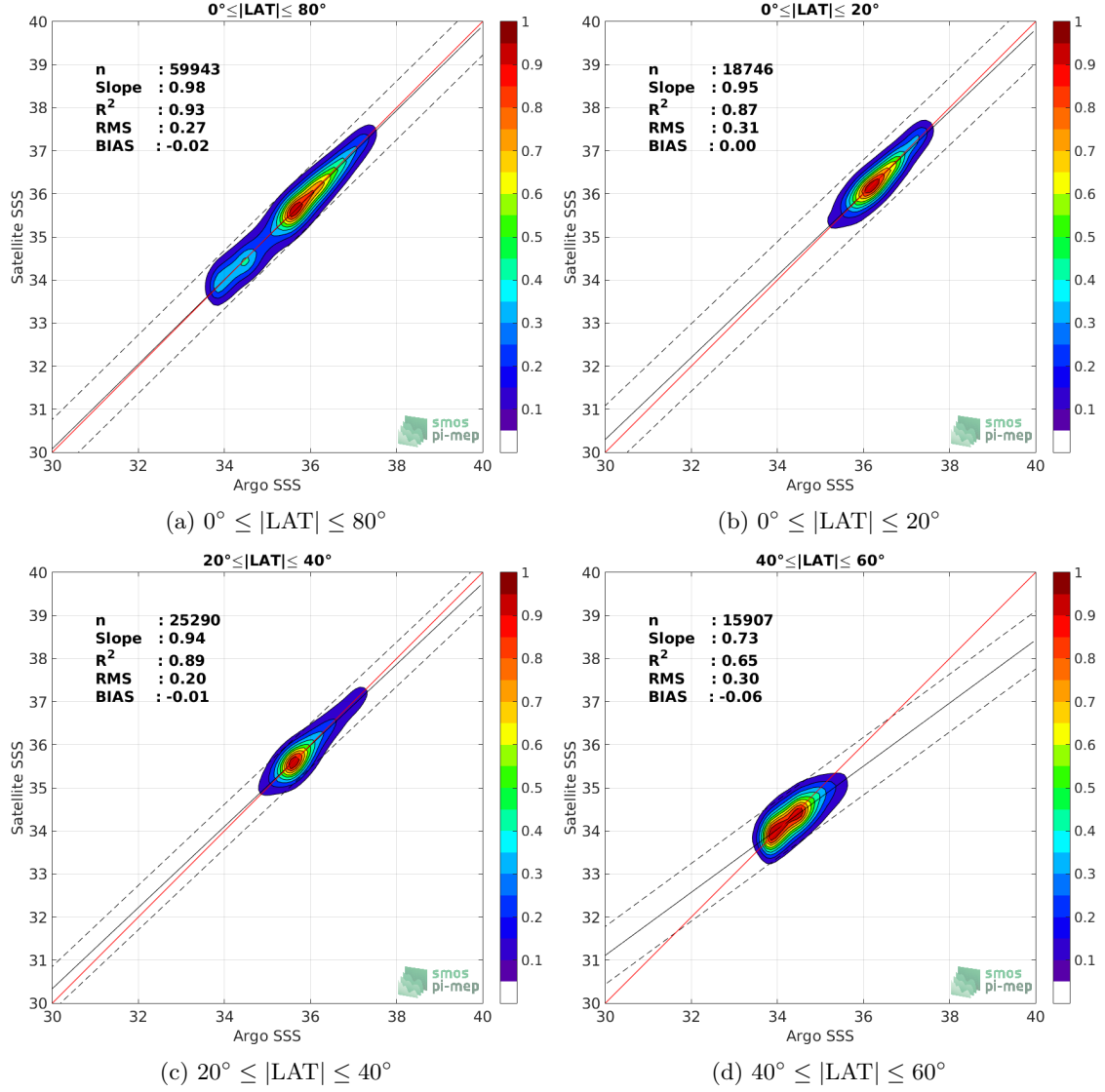
Figure 9: Contour maps of the concentration of SMAP-L3-RSS-V4-MONTHLY SSS (y-axis) versus Argo SSS (x-axis) at match-up pairs for different latitude bands. For each plot, the red line shows x=y . The black thin and dashed lines indicate a linear fit through the data cloud and the \pm 95\% confidence levels, respectively. The number match-up pairs n , the slope and R^2 coefficient of the linear fit, the root mean square (RMS) and the mean bias between satellite and in situ data are indicated for each latitude band in each plots.
