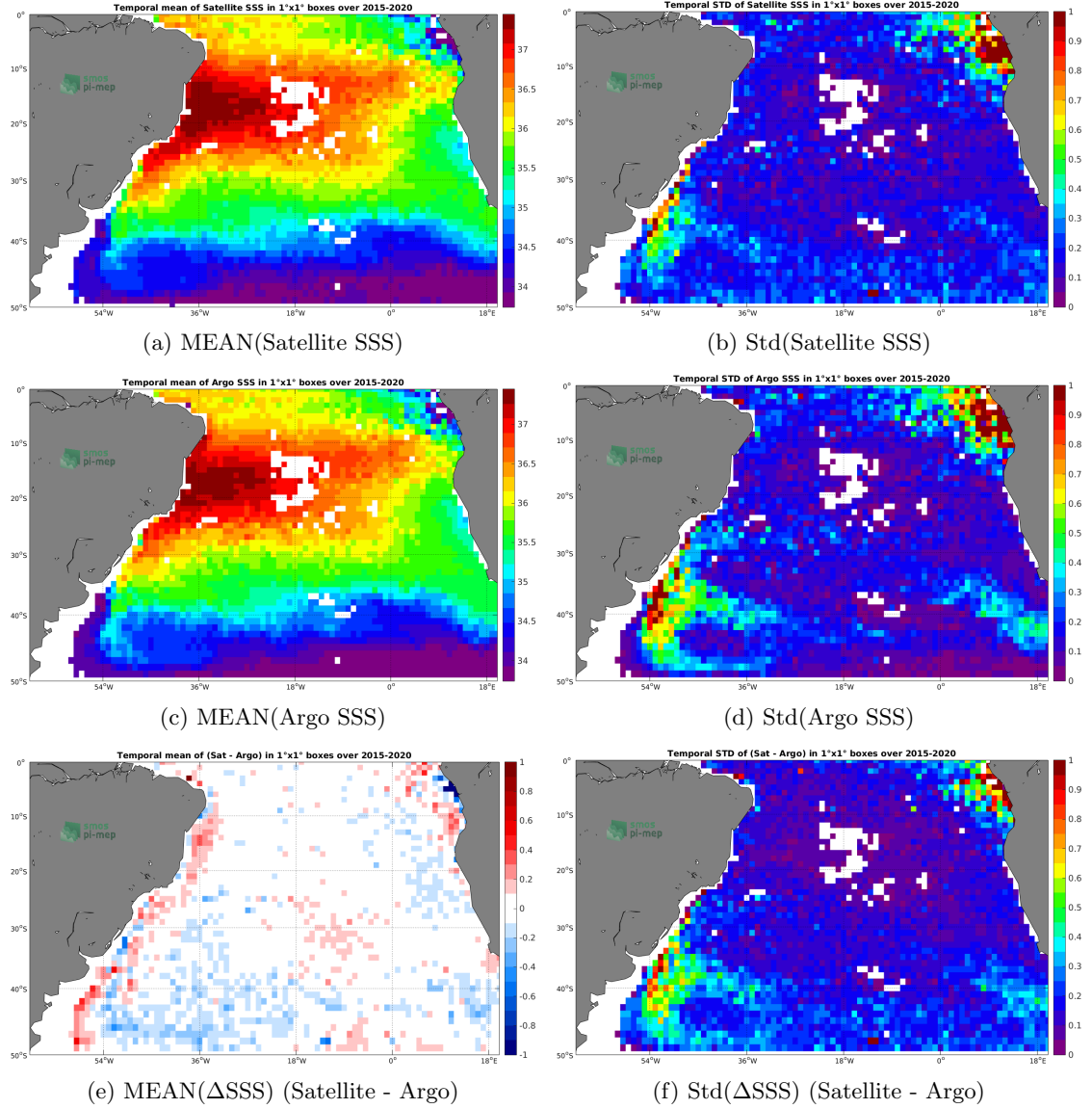
Figure 6: Temporal mean (left) and Std (right) of SSS from SMAP-L3-RSS-V4-MONTHLY (top), Argo (middle), and of \Delta SSS (Satellite - Argo). Only match-up pairs are used to generate these maps.
