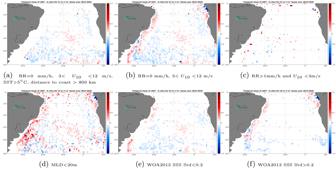
Figure 12: Temporal mean gridded over spatial boxes of size 1^\circ \times 1^\circ of \Delta SSS (SMAP-L3-RSS-V4-MONTHLY - Argo) for 6 different subdatasets corresponding to: RR=0 mm/h, 3 < U_{10} < 12 m/s, SST > 5^\circ\text{C} , distance to coast > 800 km (a), RR=0 mm/h, 3 < U_{10} < 12 m/s (b), RR > 1 mm/h and U_{10} < 4 m/s (c), MLD < 20 m (d), WOA2013 SSS Std < 0.2 (e), WOA2013 SSS Std > 0.2 (f).
