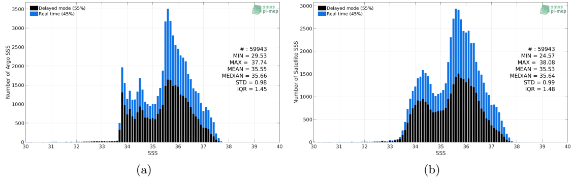
Figure 2: Histograms of SSS from Argo (a) and SMAP-L3-RSS-V4-MONTHLY (b) considering all match-up pairs per bins of 0.1 over the South Atlantic Ocean Pi-MEP region and for the full satellite product period.
