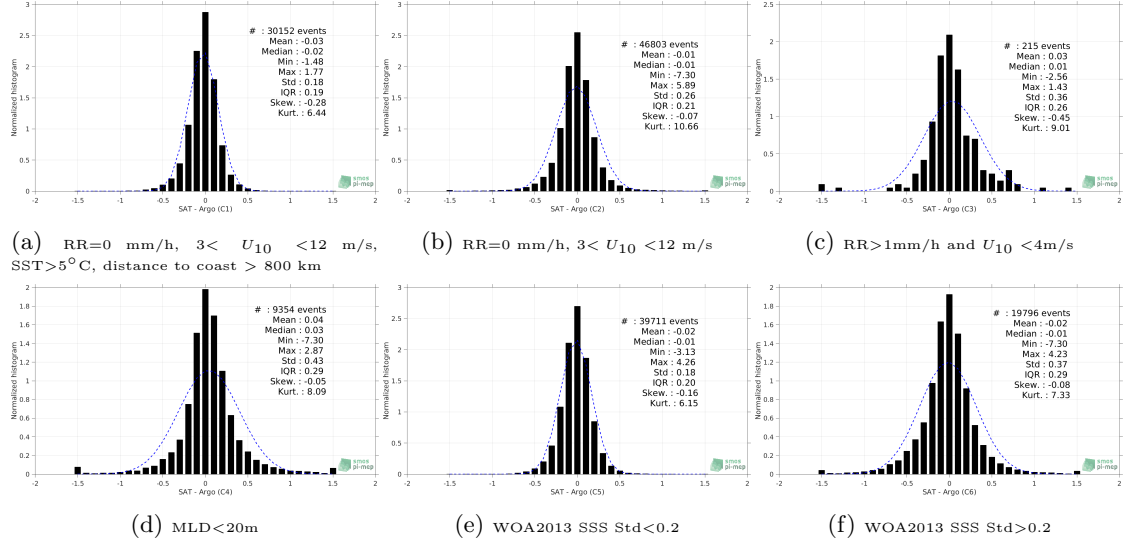
Figure 13: Normalized histogram of \Delta SSS (SMAP-L3-RSS-V4-MONTHLY - Argo) for 6 different subdatasets corresponding to: RR=0 mm/h, 3 < U_{10} < 12 m/s, SST>5°C, distance to coast > 800 km (a), RR=0 mm/h, 3 < U_{10} < 12 m/s (b), RR>1mm/h and U_{10} < 4 m/s (c), MLD<20m (d), WOA2013 SSS Std<0.2 (e), WOA2013 SSS Std>0.2 (f).
