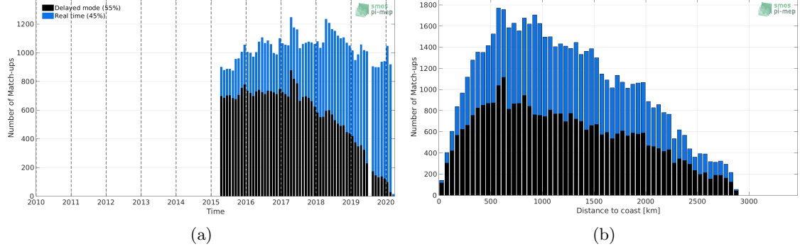
Figure 1: Number of match-ups between Argo and SMAP-L3-RSS-V4-MONTHLY SSS as a function of time (a) and as function of the distance to coast (b) over the South Atlantic Ocean Pi-MEP region and for the full satellite product period.
