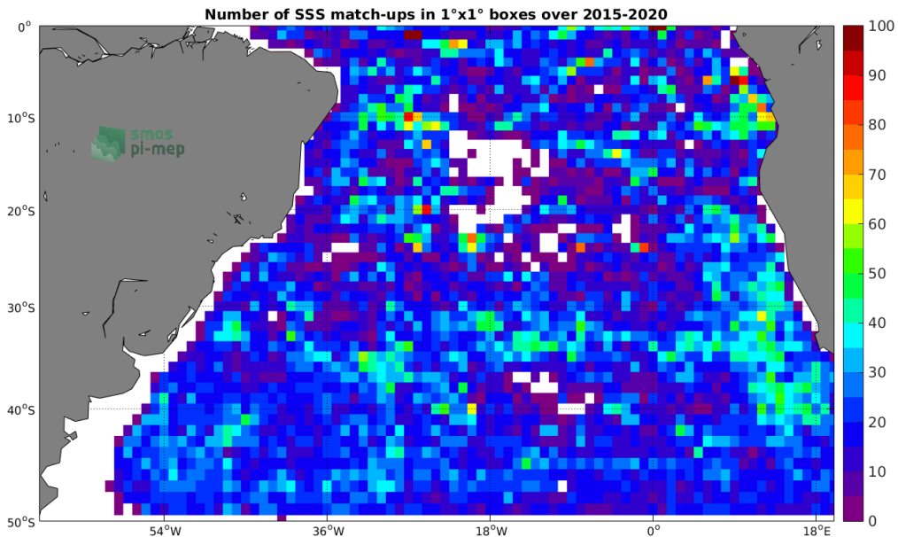
Figure 4: Number of SSS match-ups between Argo SSS and the SMAP-L3-RSS-V4-MONTHLY SSS product for the South Atlantic Ocean Pi-MEP region over 1°x1° boxes and for the full satellite product period.
