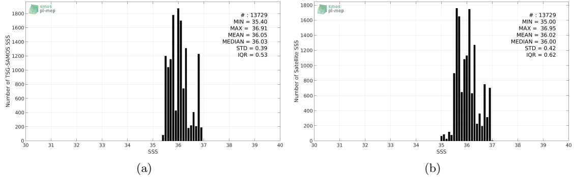
Figure 2: Histograms of SSS from TSG-SAMOS (a) and SMAP-L3-RSS-V3-8DAY-RUNNING-70KM (b) considering all match-up pairs per bins of 0.1 over the South Atlantic Ocean Pi-MEP region and for the full satellite product period.
