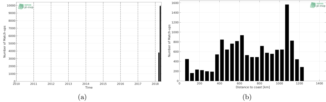
Figure 1: Number of match-ups between TSG-SAMOS and SMAP-L3-RSS-V3-8DAY-RUNNING-70KM SSS as a function of time (a) and as function of the distance to coast (b) over the South Atlantic Ocean Pi-MEP region and for the full satellite product period.
