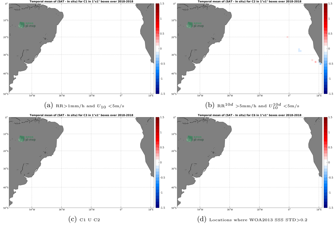
Figure 12: Temporal mean gridded over spatial boxes of size 1^\circ \times 1^\circ of \Delta SSS (SMAP-L3-RSS-V3-8DAY-RUNNING-70KM - TSG-SAMOS) for 4 different subdatasets corresponding to: RR > 1mm/h and U_{10} < 5\text{m/s} (a), RR^{10d} > 5\text{mm/h} and U_{10}^{10d} < 5\text{m/s} (b), C1 U C2 (c), Locations where WOA2013 SSS STD > 0.2 (d).
