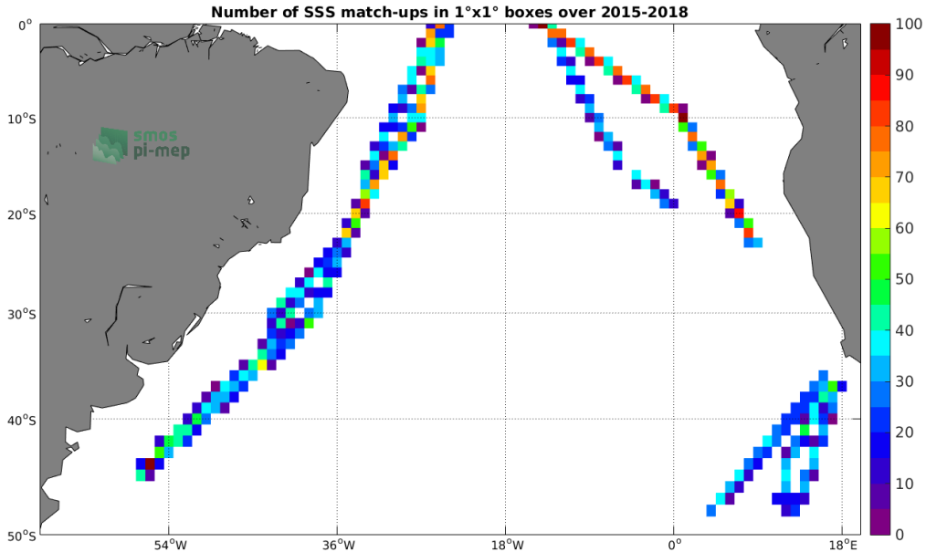
Figure 4: Number of SSS match-ups between TSG-POLARSTERN SSS and the SMAP-L3-RSS-V3-8DAY-RUNNING-70KM SSS product for the South Atlantic Ocean Pi-MEP region over 1^\circ \times 1^\circ boxes and for the full satellite product period.
