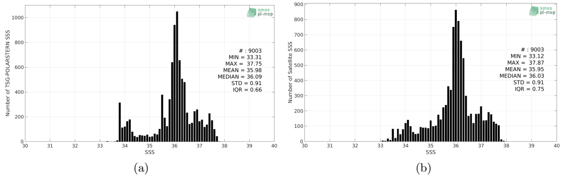
Figure 2: Histograms of SSS from TSG-POLARSTERN (a) and SMAP-L3-RSS-V3-8DAY-RUNNING-70KM (b) considering all match-up pairs per bins of 0.1 over the South Atlantic Ocean Pi-MEP region and for the full satellite product period.
