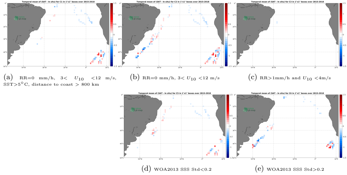
Figure 12: Temporal mean gridded over spatial boxes of size 1^\circ \times 1^\circ of \Delta SSS (SMAP-L3-RSS-V3-8DAY-RUNNING-70KM - TSG-POLARSTERN) for 5 different subdatasets corresponding to: RR=0 mm/h, 3 < U_{10} < 12 m/s, SST > 5^\circ\text{C} , distance to coast > 800 km (a), RR=0 mm/h, 3 < U_{10} < 12 m/s (b), RR > 1 mm/h and U_{10} < 4 m/s (c), WOA2013 SSS Std < 0.2 (d), WOA2013 SSS Std > 0.2 (e).
