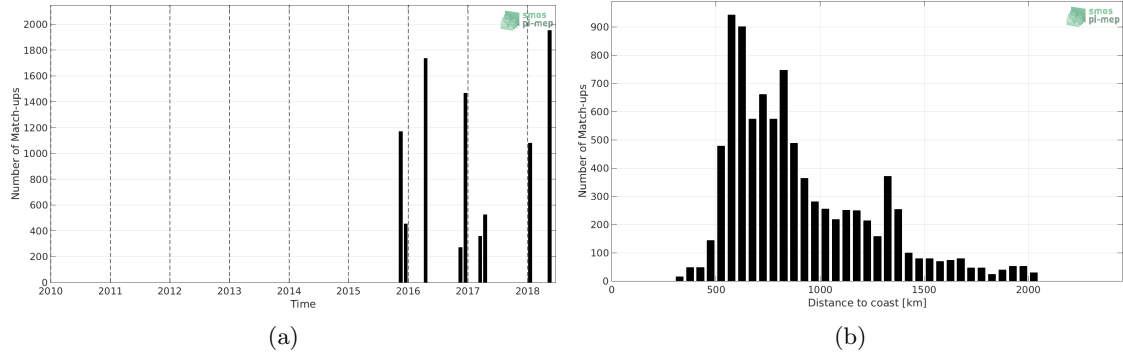
Figure 1: Number of match-ups between TSG-POLARSTERN and SMAP-L3-RSS-V3-8DAY-RUNNING-70KM SSS as a function of time (a) and as function of the distance to coast (b) over the South Atlantic Ocean Pi-MEP region and for the full satellite product period.
