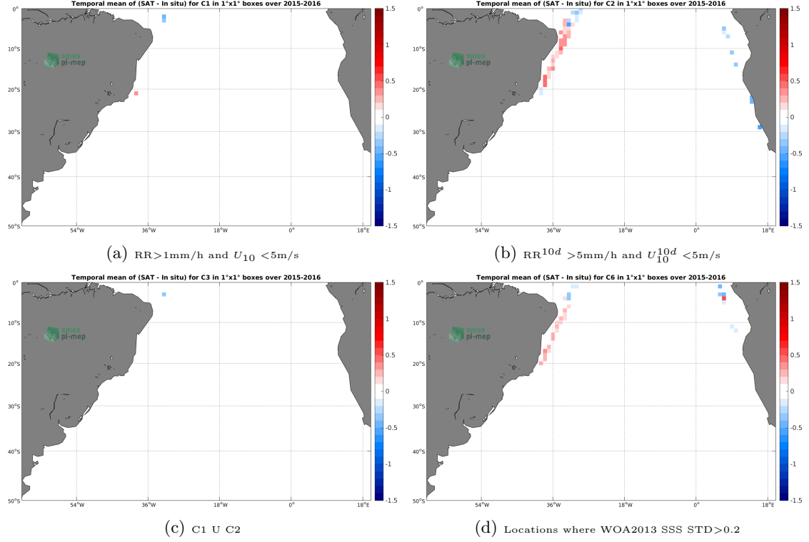
Figure 12: Temporal mean gridded over spatial boxes of size 1^\circ \times 1^\circ of \Delta SSS (SMAP-L3-RSS-V3-8DAY-RUNNING-70KM - TSG-LEGOS-DM) for 4 different subdatasets corresponding to: RR > 1mm/h and U_{10} < 5\text{m/s} (a), RR^{10d} > 5\text{mm/h} and U_{10}^{10d} < 5\text{m/s} (b), C1 U C2 (c), Locations where WOA2013 SSS STD > 0.2 (d).
