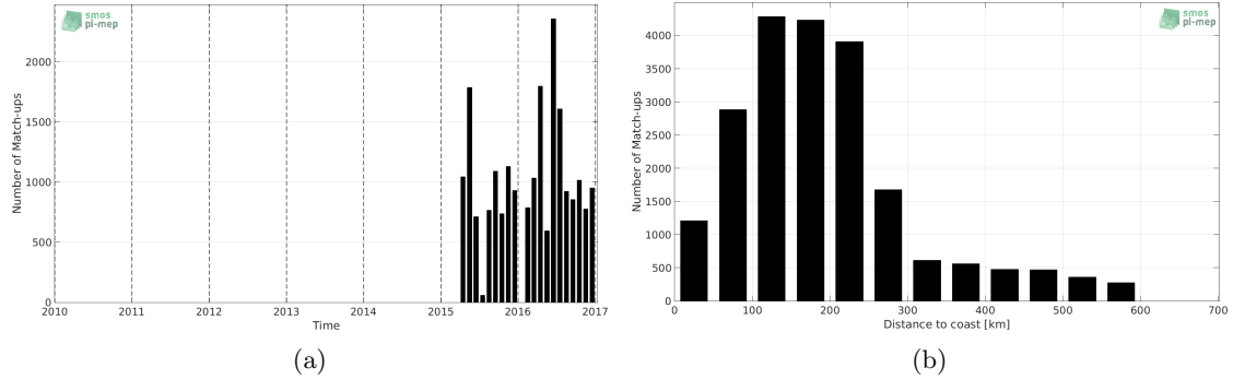
Figure 1: Number of match-ups between TSG-LEGOS-DM and SMAP-L3-RSS-V3-8DAY-RUNNING-70KM SSS as a function of time (a) and as function of the distance to coast (b) over the South Atlantic Ocean Pi-MEP region and for the full satellite product period.
