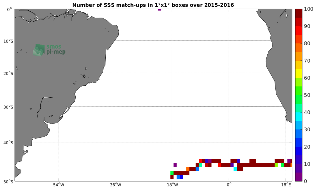
Figure 3: Number of SSS match-ups between Surface drifters SSS and the SMAP-L3-RSS-V3-8DAY-RUNNING-70KM SSS product for the South Atlantic Ocean Pi-MEP region over 1°x1° boxes and for the full satellite product period.
