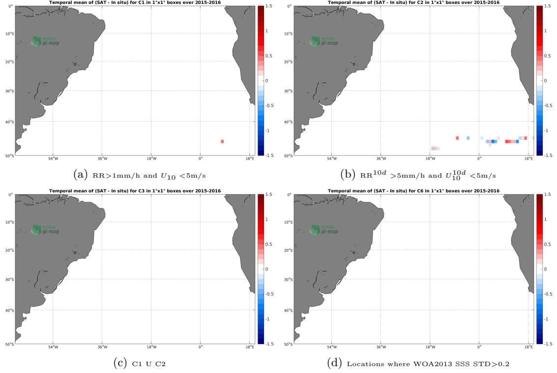
Figure 11: Temporal mean gridded over spatial boxes of size 1^\circ \times 1^\circ of \Delta SSS (SMAP-L3-RSS-V3-8DAY-RUNNING-70KM - Surface drifters) for 4 different subdatasets corresponding to: RR > 1\text{mm/h} and U_{10} < 5\text{m/s} (a), RR^{10d} > 5\text{mm/h} and U_{10}^{10d} < 5\text{m/s} (b), C1 U C2 (c), Locations where WOA2013 SSS STD > 0.2 (d).
