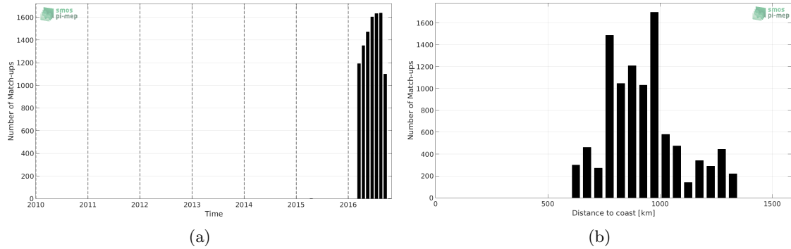
Figure 1: Number of match-ups between Surface drifters and SMAP-L3-RSS-V3-8DAY-RUNNING-70KM SSS as a function of time (a) and as function of the distance to coast (b) over the South Atlantic Ocean Pi-MEP region and for the full satellite product period.
