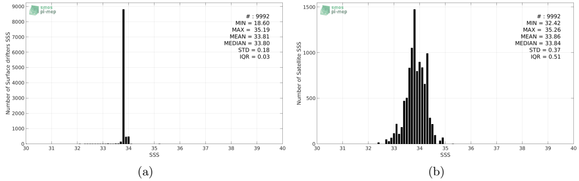
Figure 2: Histograms of SSS from Surface drifters (a) and SMAP-L3-RSS-V3-8DAY-RUNNING-70KM (b) considering all match-up pairs per bins of 0.1 over the South Atlantic Ocean Pi-MEP region and for the full satellite product period.
