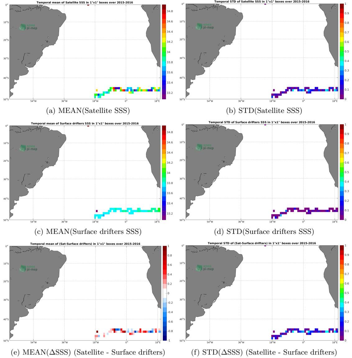
Figure 5: Temporal mean (left) and STD (right) of SSS from SMAP-L3-RSS-V3-8DAY-RUNNING-70KM (top), Surface drifters (middle), and of \Delta SSS (Satellite - Surface drifters). Only match-up pairs are used to generate these maps.
