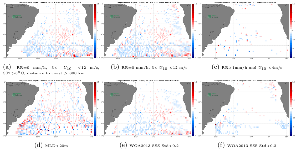
Figure 12: Temporal mean gridded over spatial boxes of size 1^\circ \times 1^\circ of \Delta SSS (SMAP-L3-RSS-V3-8DAY-RUNNING-70KM - Argo) for 6 different subdatasets corresponding to: RR=0 mm/h, 3 < U_{10} < 12 m/s, SST > 5^\circ C , distance to coast > 800 km (a), RR=0 mm/h, 3 < U_{10} < 12 m/s (b), RR > 1 mm/h and U_{10} < 4 m/s (c), MLD < 20 m (d), WOA2013 SSS Std < 0.2 (e), WOA2013 SSS Std > 0.2 (f).
