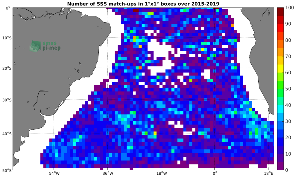
Figure 4: Number of SSS match-ups between Argo SSS and the SMAP-L3-RSS-V3-8DAY-RUNNING-70KM SSS product for the South Atlantic Ocean Pi-MEP region over 1^\circ \times 1^\circ boxes and for the full satellite product period.
