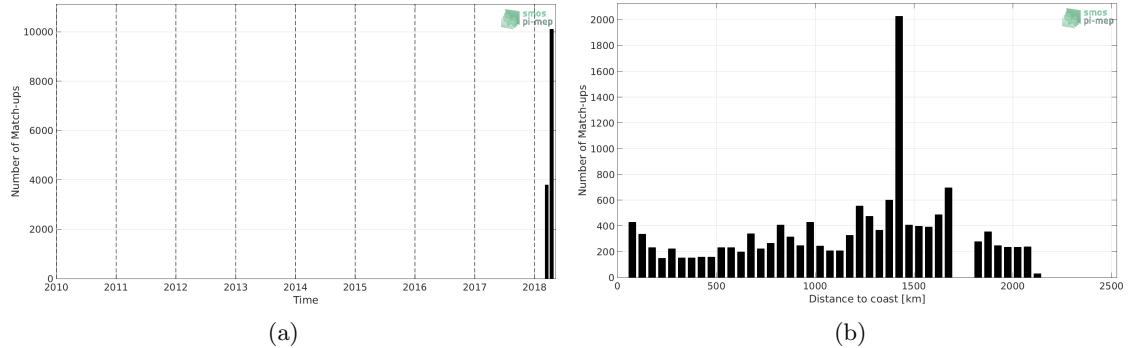
Figure 1: Number of match-ups between TSG-SAMOS and SMAP-L3-RSS-V3-8DAY-RUNNING-40KM SSS as a function of time (a) and as function of the distance to coast (b) over the South Atlantic Ocean Pi-MEP region and for the full satellite product period.
