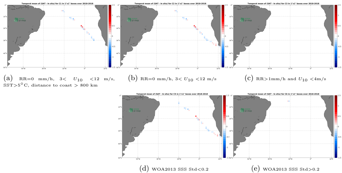
Figure 12: Temporal mean gridded over spatial boxes of size 1^\circ \times 1^\circ of \Delta SSS (SMAP-L3-RSS-V3-8DAY-RUNNING-40KM - TSG-SAMOS) for 5 different subdatasets corresponding to: RR=0 mm/h, 3 < U_{10} < 12 m/s, SST > 5^\circ C , distance to coast > 800 km (a), RR=0 mm/h, 3 < U_{10} < 12 m/s (b), RR > 1 mm/h and U_{10} < 4 m/s (c), WOA2013 SSS Std < 0.2 (d), WOA2013 SSS Std > 0.2 (e).
