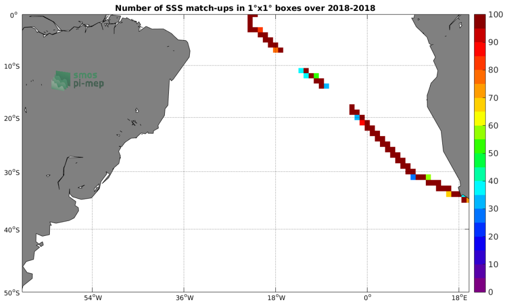
Figure 4: Number of SSS match-ups between TSG-SAMOS SSS and the SMAP-L3-RSS-V3-8DAY-RUNNING-40KM SSS product for the South Atlantic Ocean Pi-MEP region over 1^\circ \times 1^\circ boxes and for the full satellite product period.
