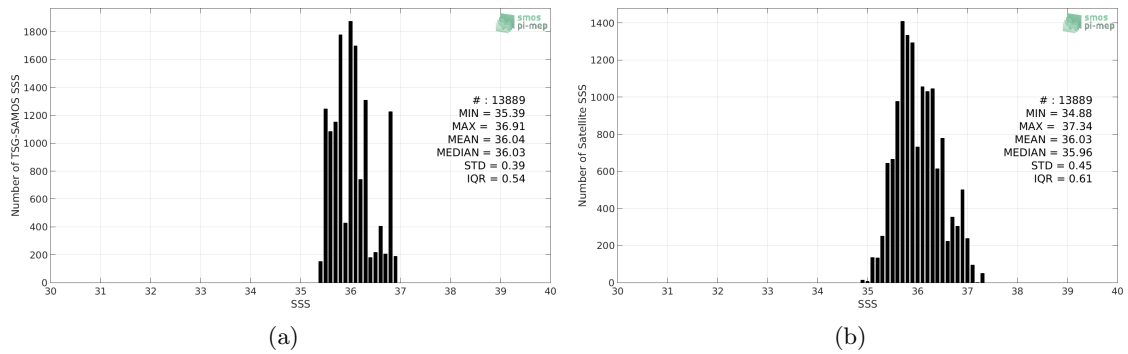
Figure 2: Histograms of SSS from TSG-SAMOS (a) and SMAP-L3-RSS-V3-8DAY-RUNNING-40KM (b) considering all match-up pairs per bins of 0.1 over the South Atlantic Ocean Pi-MEP region and for the full satellite product period.
