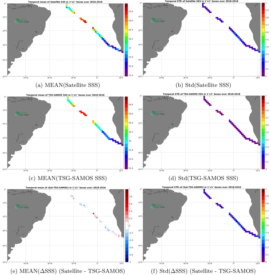
Figure 6: Temporal mean (left) and Std (right) of SSS from SMAP-L3-RSS-V3-8DAY-RUNNING-40KM (top), TSG-SAMOS (middle), and of \Delta SSS (Satellite - TSG-SAMOS). Only match-up pairs are used to generate these maps.
