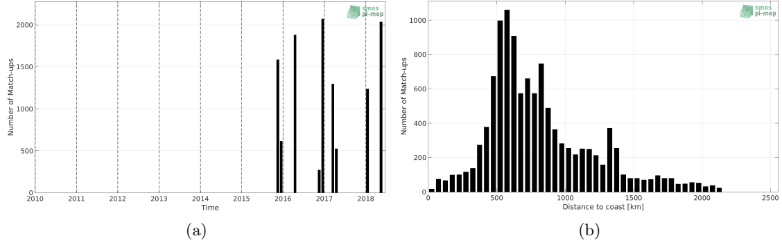
Figure 1: Number of match-ups between TSG-POLARSTERN and SMAP-L3-RSS-V3-8DAY-RUNNING-40KM SSS as a function of time (a) and as function of the distance to coast (b) over the South Atlantic Ocean Pi-MEP region and for the full satellite product period.
