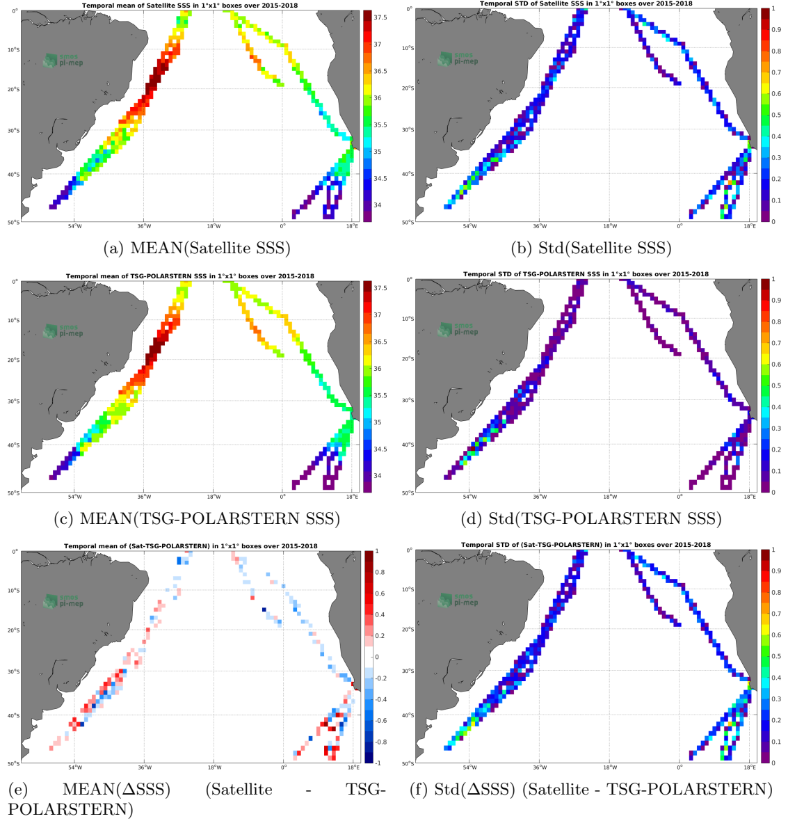
Figure 6: Temporal mean (left) and Std (right) of SSS from SMAP-L3-RSS-V3-8DAY-RUNNING-40KM (top), TSG-POLARSTERN (middle), and of \Delta SSS (Satellite - TSG-POLARSTERN). Only match-up pairs are used to generate these maps.
