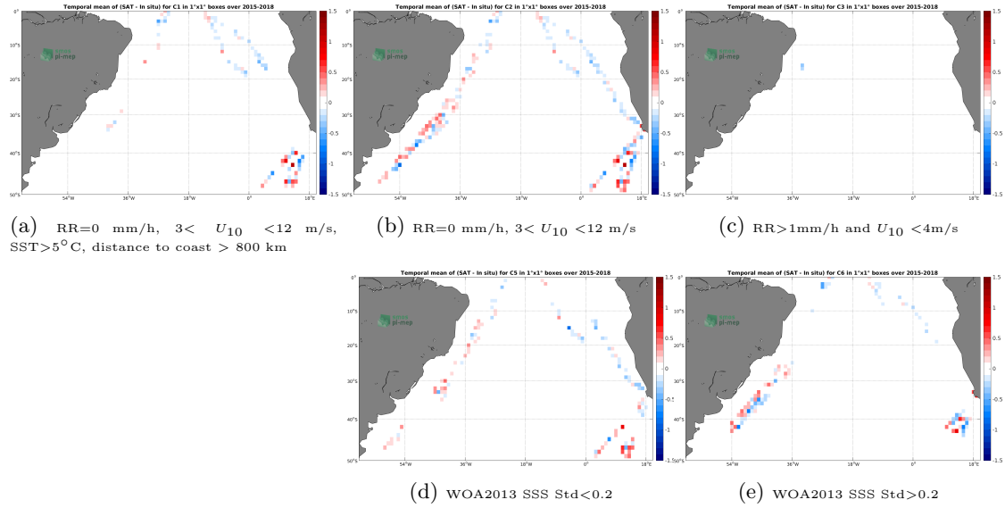
Figure 12: Temporal mean gridded over spatial boxes of size 1^\circ \times 1^\circ of \Delta SSS (SMAP-L3-RSS-V3-8DAY-RUNNING-40KM - TSG-POLARSTERN) for 5 different subdatasets corresponding to: RR=0 mm/h, 3 < U_{10} < 12 m/s, SST > 5^\circ\text{C} , distance to coast > 800 km (a), RR=0 mm/h, 3 < U_{10} < 12 m/s (b), RR > 1 mm/h and U_{10} < 4 m/s (c), WOA2013 SSS Std < 0.2 (d), WOA2013 SSS Std > 0.2 (e).
