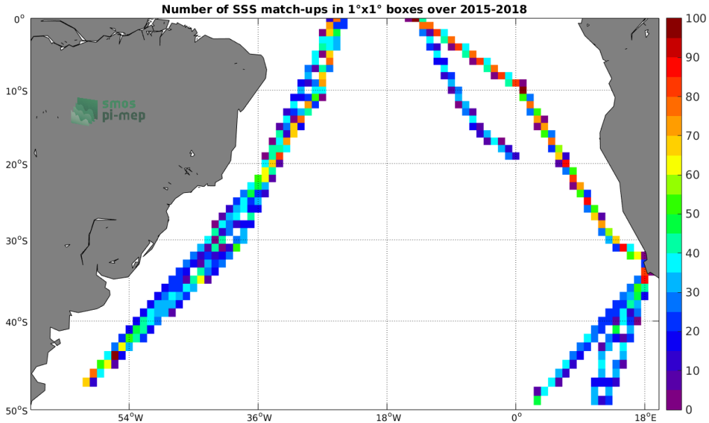
Figure 4: Number of SSS match-ups between TSG-POLARSTERN SSS and the SMAP-L3-RSS-V3-8DAY-RUNNING-40KM SSS product for the South Atlantic Ocean Pi-MEP region over 1^\circ \times 1^\circ boxes and for the full satellite product period.
