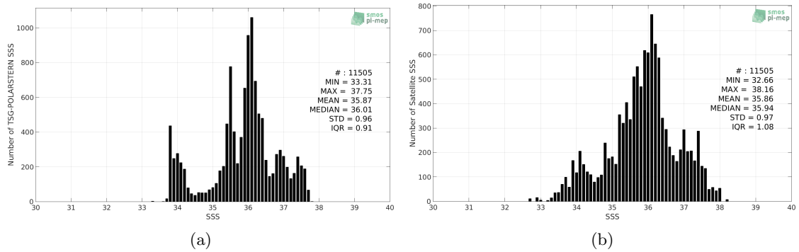
Figure 2: Histograms of SSS from TSG-POLARSTERN (a) and SMAP-L3-RSS-V3-8DAY-RUNNING-40KM (b) considering all match-up pairs per bins of 0.1 over the South Atlantic Ocean Pi-MEP region and for the full satellite product period.
