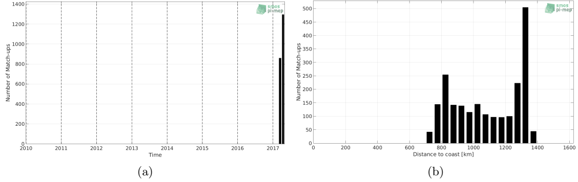
Figure 1: Number of match-ups between TSG-GOSUD-Sailing-ship and SMAP-L3-RSS-V3-8DAY-RUNNING-40KM SSS as a function of time (a) and as function of the distance to coast (b) over the South Atlantic Ocean Pi-MEP region and for the full satellite product period.
