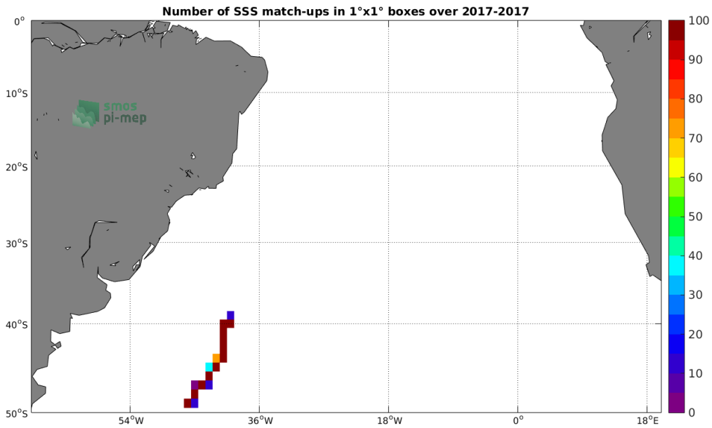
Figure 4: Number of SSS match-ups between TSG-GOSUD-Sailing-ship SSS and the SMAP-L3-RSS-V3-8DAY-RUNNING-40KM SSS product for the South Atlantic Ocean Pi-MEP region over 1^\circ \times 1^\circ boxes and for the full satellite product period.
