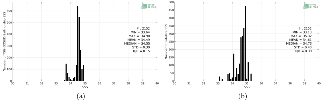
Figure 2: Histograms of SSS from TSG-GOSUD-Sailing-ship (a) and SMAP-L3-RSS-V3-8DAY-RUNNING-40KM (b) considering all match-up pairs per bins of 0.1 over the South Atlantic Ocean Pi-MEP region and for the full satellite product period.
