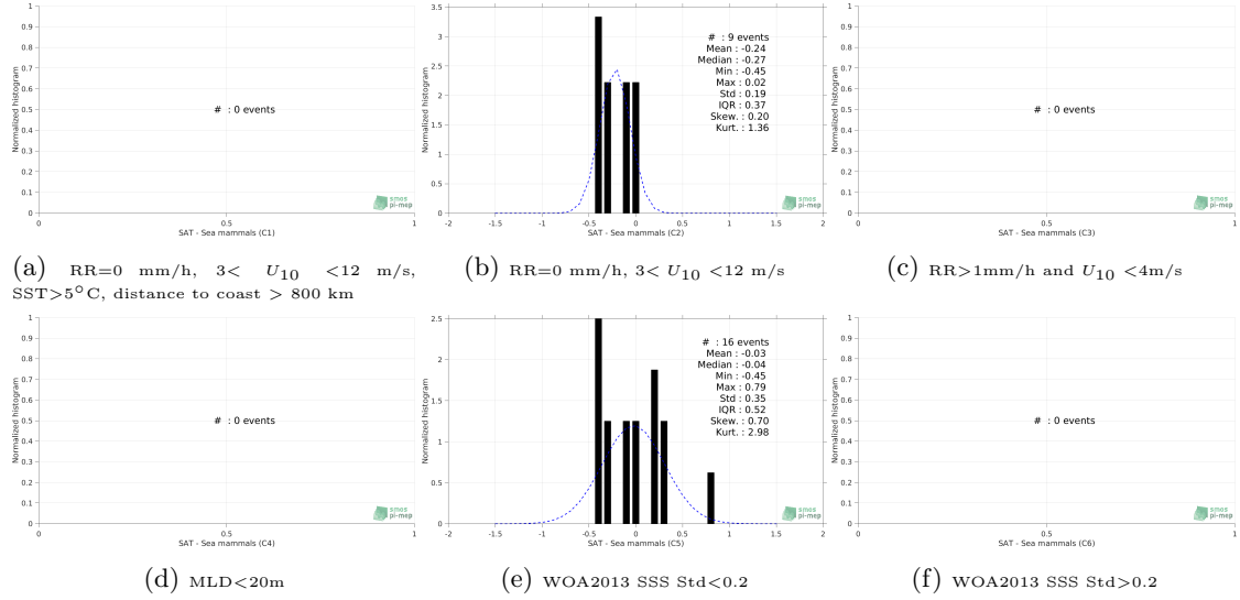
Figure 13: Normalized histogram of \Delta\text{SSS} (SMAP-L3-RSS-V3-8DAY-RUNNING-40KM - Sea mammals) for 6 different subdatasets corresponding to: RR=0 mm/h, 3 < U_{10} < 12 m/s, SST > 5^\circ\text{C} , distance to coast > 800 km (a), RR=0 mm/h, 3 < U_{10} < 12 m/s (b), RR > 1 mm/h and U_{10} < 4 m/s (c), MLD < 20 m (d), WOA2013 SSS Std < 0.2 (e), WOA2013 SSS Std > 0.2 (f).
