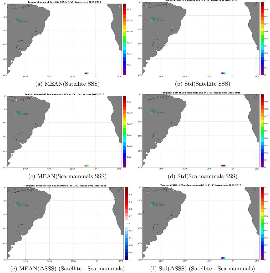
Figure 6: Temporal mean (left) and Std (right) of SSS from SMAP-L3-RSS-V3-8DAY-RUNNING-40KM (top), Sea mammals (middle), and of \Delta SSS (Satellite - Sea mammals). Only match-up pairs are used to generate these maps.
