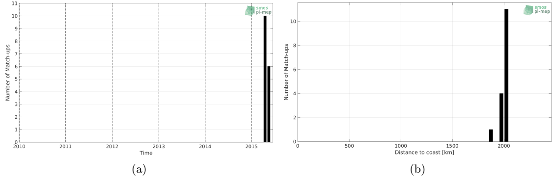
Figure 1: Number of match-ups between Sea mammals and SMAP-L3-RSS-V3-8DAY-RUNNING-40KM SSS as a function of time (a) and as function of the distance to coast (b) over the South Atlantic Ocean Pi-MEP region and for the full satellite product period.
