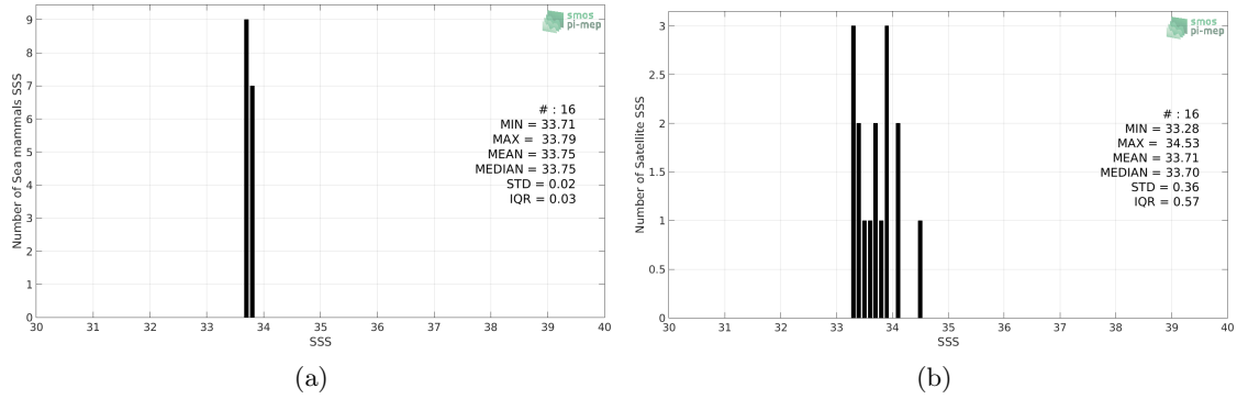
Figure 2: Histograms of SSS from Sea mammals (a) and SMAP-L3-RSS-V3-8DAY-RUNNING-40KM (b) considering all match-up pairs per bins of 0.1 over the South Atlantic Ocean Pi-MEP region and for the full satellite product period.
