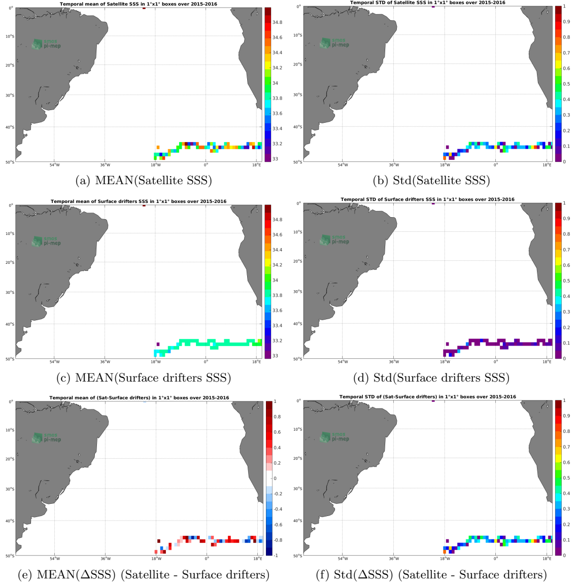
Figure 5: Temporal mean (left) and Std (right) of SSS from SMAP-L3-RSS-V3-8DAY-RUNNING-40KM (top), Surface drifters (middle), and of \Delta SSS (Satellite - Surface drifters). Only match-up pairs are used to generate these maps.
