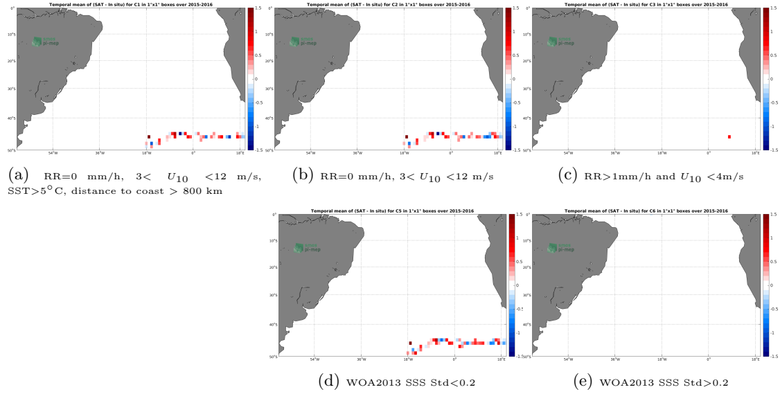
Figure 11: Temporal mean gridded over spatial boxes of size 1^\circ \times 1^\circ of \Delta SSS (SMAP-L3-RSS-V3-8DAY-RUNNING-40KM - Surface drifters) for 5 different subdatasets corresponding to: RR=0 mm/h, 3 < U_{10} < 12 m/s, SST > 5^\circ C , distance to coast > 800 km (a), RR=0 mm/h, 3 < U_{10} < 12 m/s (b), RR > 1 mm/h and U_{10} < 4 m/s (c), WOA2013 SSS Std < 0.2 (d), WOA2013 SSS Std > 0.2 (e).
