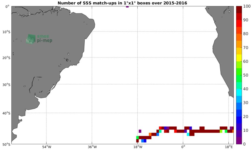
Figure 3: Number of SSS match-ups between Surface drifters SSS and the SMAP-L3-RSS-V3-8DAY-RUNNING-40KM SSS product for the South Atlantic Ocean Pi-MEP region over 1^\circ \times 1^\circ boxes and for the full satellite product period.
