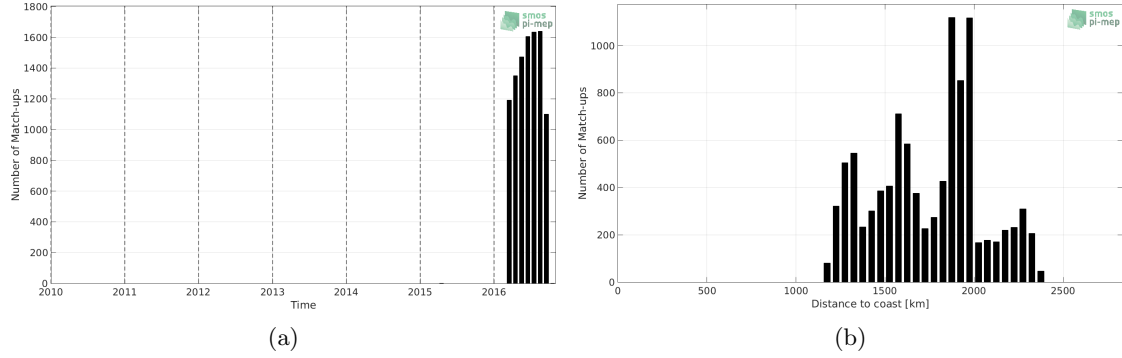
Figure 1: Number of match-ups between Surface drifters and SMAP-L3-RSS-V3-8DAY-RUNNING-40KM SSS as a function of time (a) and as function of the distance to coast (b) over the South Atlantic Ocean Pi-MEP region and for the full satellite product period.
