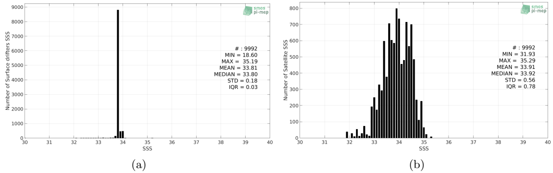
Figure 2: Histograms of SSS from Surface drifters (a) and SMAP-L3-RSS-V3-8DAY-RUNNING-40KM (b) considering all match-up pairs per bins of 0.1 over the South Atlantic Ocean Pi-MEP region and for the full satellite product period.
