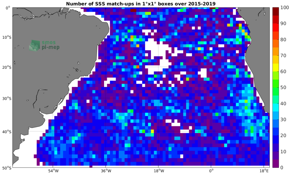
Figure 4: Number of SSS match-ups between Argo SSS and the SMAP-L3-RSS-V3-8DAY-RUNNING-40KM SSS product for the South Atlantic Ocean Pi-MEP region over 1^\circ \times 1^\circ boxes and for the full satellite product period.
