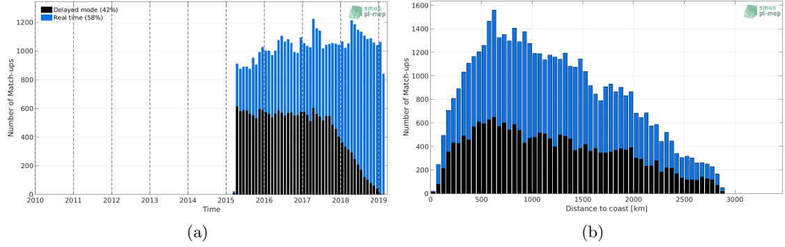
Figure 1: Number of match-ups between Argo and SMAP-L3-RSS-V3-8DAY-RUNNING-40KM SSS as a function of time (a) and as function of the distance to coast (b) over the South Atlantic Ocean Pi-MEP region and for the full satellite product period.
