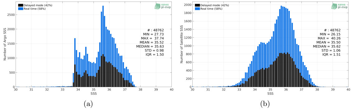
Figure 2: Histograms of SSS from Argo (a) and SMAP-L3-RSS-V3-8DAY-RUNNING-40KM (b) considering all match-up pairs per bins of 0.1 over the South Atlantic Ocean Pi-MEP region and for the full satellite product period.
