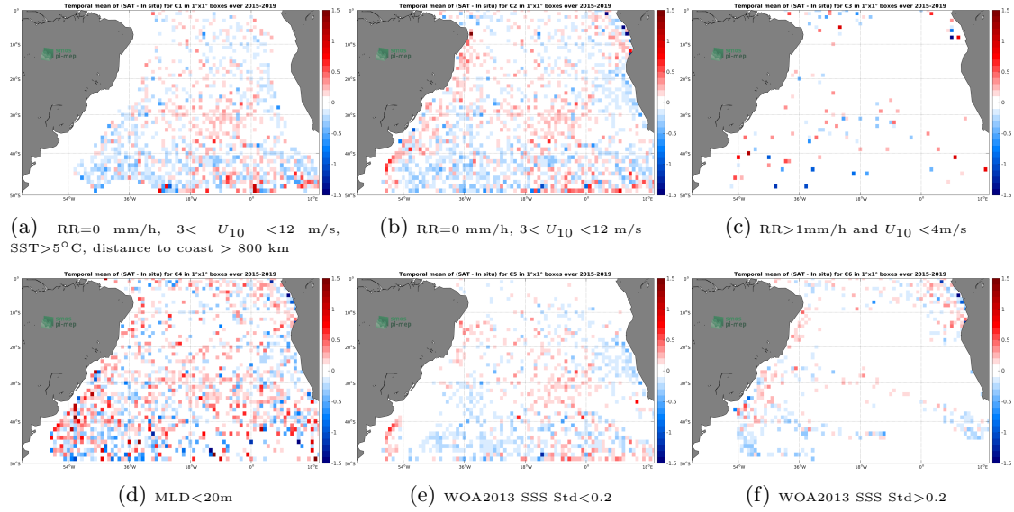
Figure 12: Temporal mean gridded over spatial boxes of size 1^\circ \times 1^\circ of \Delta SSS (SMAP-L3-RSS-V3-8DAY-RUNNING-40KM - Argo) for 6 different subdatasets corresponding to: RR=0 mm/h, 3 < U_{10} < 12 m/s, SST > 5^\circ C , distance to coast > 800 km (a), RR=0 mm/h, 3 < U_{10} < 12 m/s (b), RR > 1 mm/h and U_{10} < 4 m/s (c), MLD < 20 m (d), WOA2013 SSS Std < 0.2 (e), WOA2013 SSS Std > 0.2 (f).
