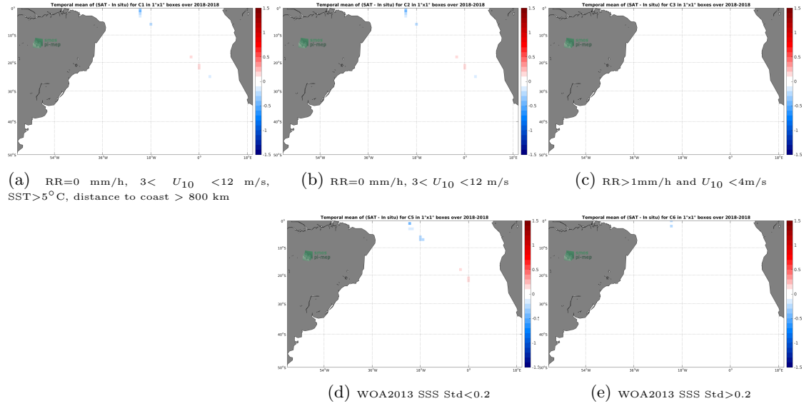
Figure 12: Temporal mean gridded over spatial boxes of size 1^\circ \times 1^\circ of \Delta SSS (SMAP-L3-RSS-V3-MONTHLY-70KM - TSG-SAMOS) for 5 different subdatasets corresponding to: RR=0 mm/h, 3 < U_{10} < 12 m/s, SST > 5^\circ\text{C} , distance to coast > 800 km (a), RR=0 mm/h, 3 < U_{10} < 12 m/s (b), RR > 1 mm/h and U_{10} < 4 m/s (c), WOA2013 SSS Std < 0.2 (d), WOA2013 SSS Std > 0.2 (e).
