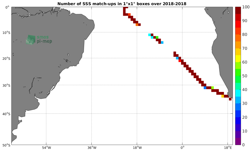
Figure 4: Number of SSS match-ups between TSG-SAMOS SSS and the SMAP-L3-RSS-V3-MONTHLY-70KM SSS product for the South Atlantic Ocean Pi-MEP region over 1^\circ \times 1^\circ boxes and for the full satellite product period.
