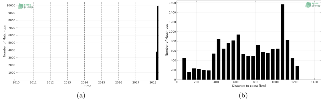
Figure 1: Number of match-ups between TSG-SAMOS and SMAP-L3-RSS-V3-MONTHLY-70KM SSS as a function of time (a) and as function of the distance to coast (b) over the South Atlantic Ocean Pi-MEP region and for the full satellite product period.
