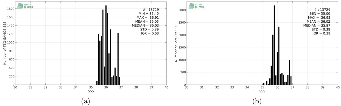
Figure 2: Histograms of SSS from TSG-SAMOS (a) and SMAP-L3-RSS-V3-MONTHLY-70KM (b) considering all match-up pairs per bins of 0.1 over the South Atlantic Ocean Pi-MEP region and for the full satellite product period.
