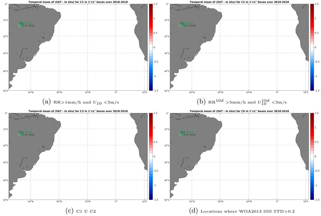
Figure 12: Temporal mean gridded over spatial boxes of size 1^\circ \times 1^\circ of \Delta SSS (SMAP-L3-RSS-V3-MONTHLY-70KM - TSG-SAMOS) for 4 different subdatasets corresponding to: RR > 1mm/h and U_{10} < 5\text{m/s} (a), RR^{10d} > 5\text{mm/h} and U_{10}^{10d} < 5\text{m/s} (b), C1 U C2 (c), Locations where WOA2013 SSS STD > 0.2 (d).
